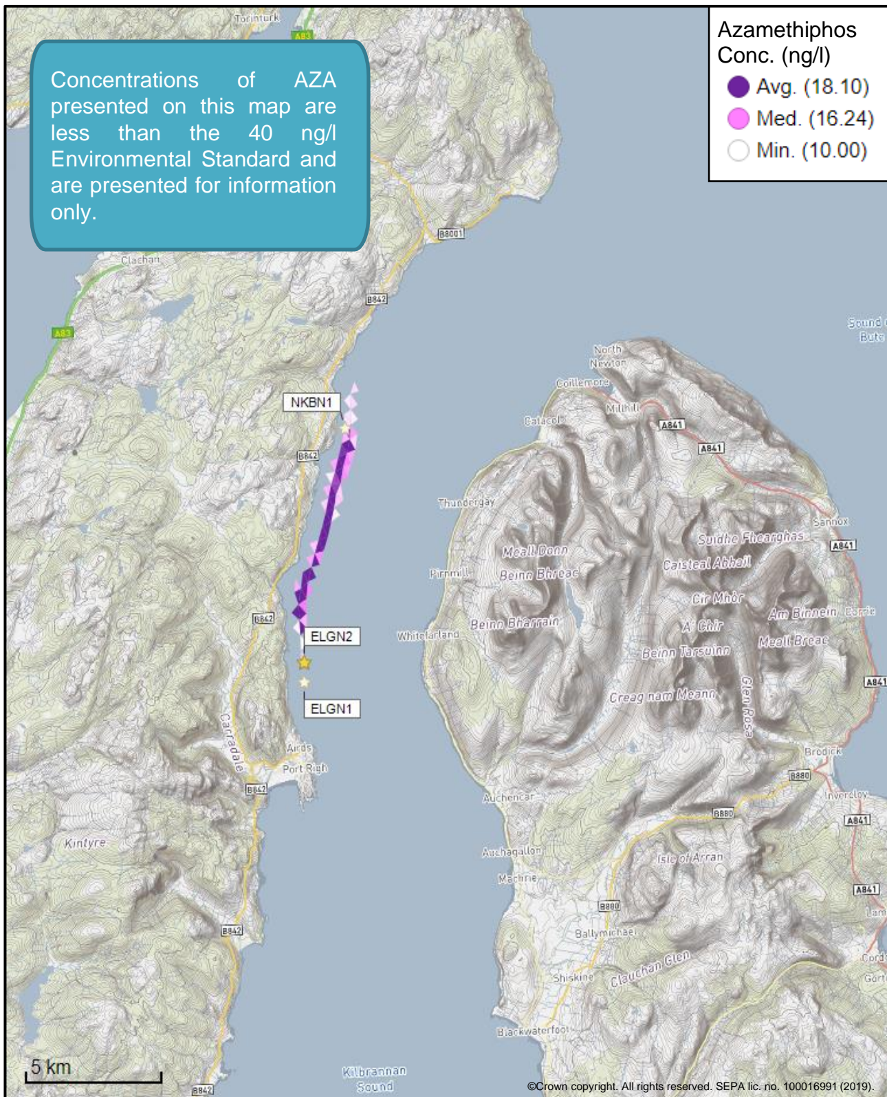
Figure 4: Modelled average Azamethiphos concentration over four days from neap tide release for the proposed site only (Carradale North (ELGN2)).
