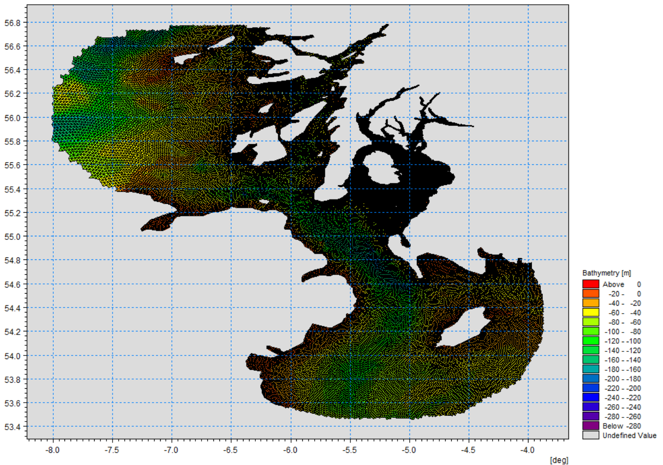
Figure 1: Firth of Clyde model grid
