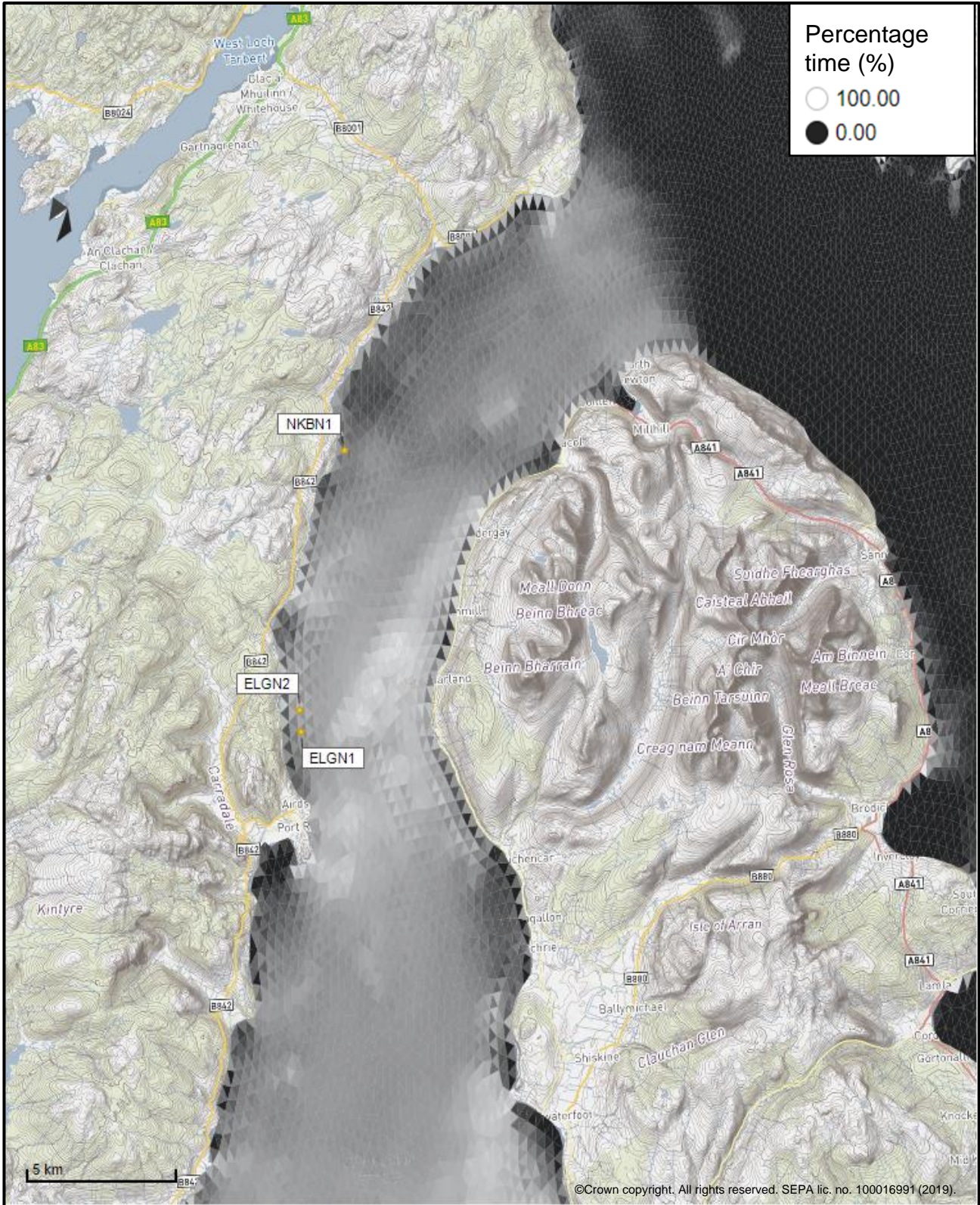
Figure 3: Modelled percentage of time the water flow speed is above 0.095 m/s in the sea area surrounding the proposed site (Carradale North (ELGN2)).
