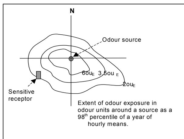
Figure 4.1 Odour contours around a source
