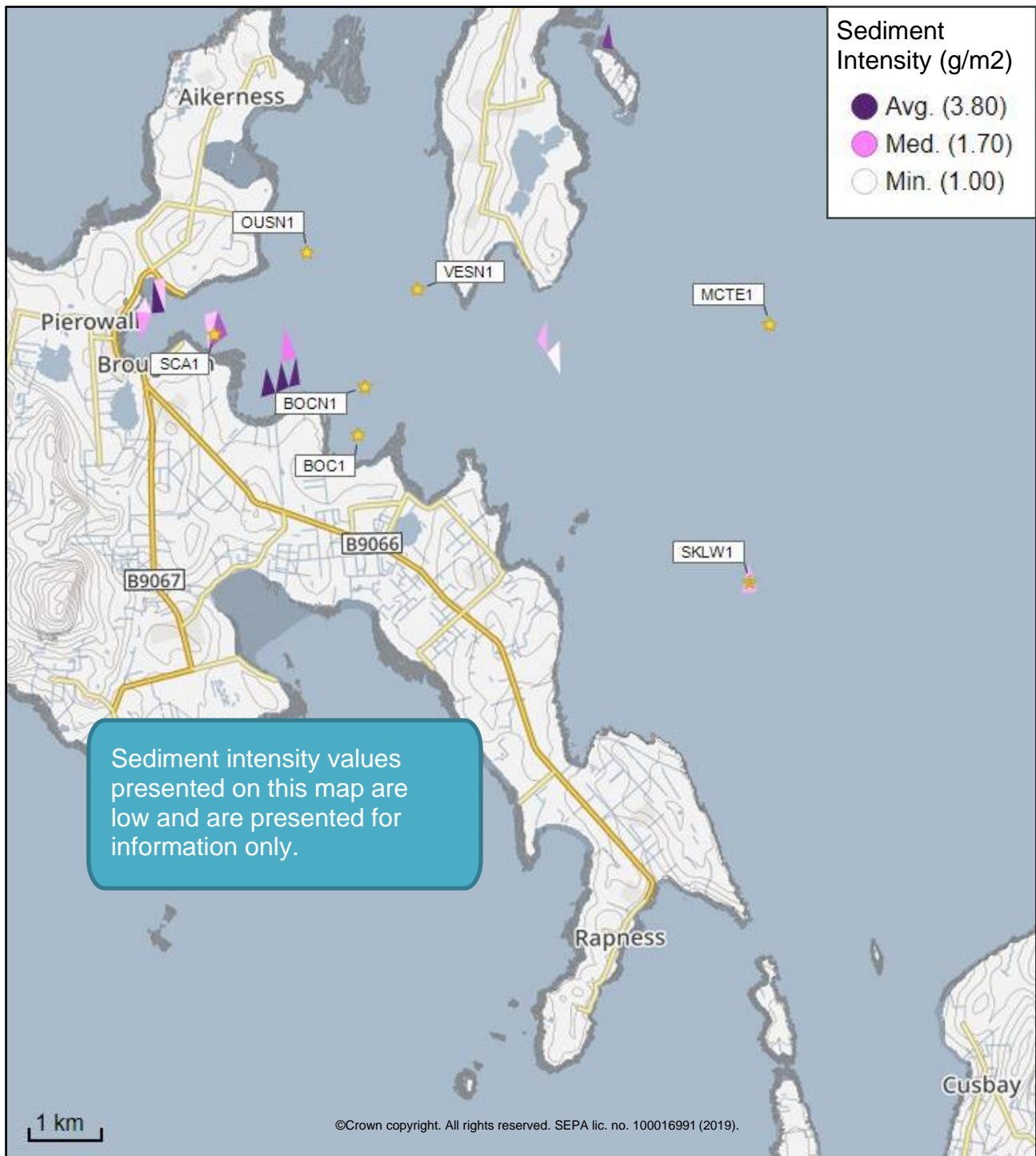
Figure 5: Modelled average sediment intensity over one month for the proposed site (East of Skelwick Skerry (SKLW1)) and other relevant sites.
