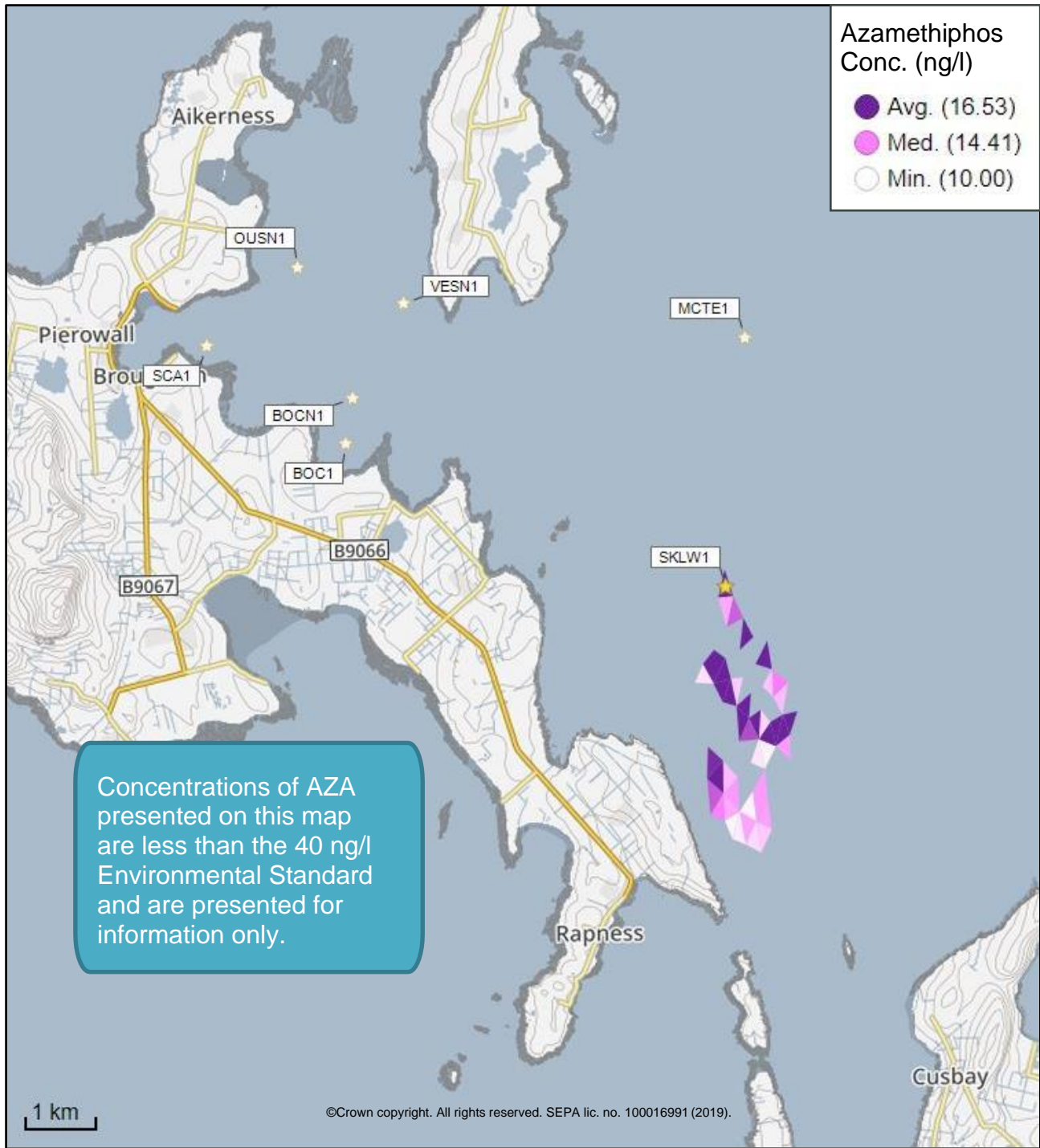
Figure 6: Modelled average Azamethiphos concentration over four days from neap tide release for the proposed site only (East of Skelwick Skerry (SKLW1)).
