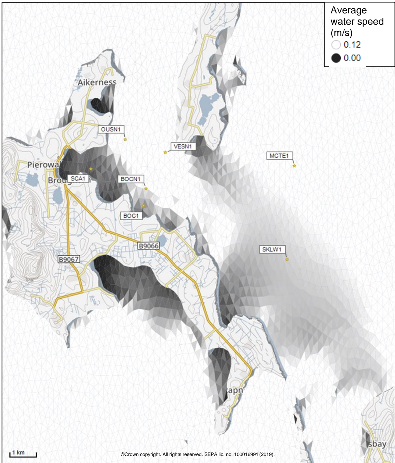
Figure 2: Modelled average water speed (metres per second – m/s) in the sea area surrounding the proposed site (East of Skelwick Skerry (SKLW1)-).
