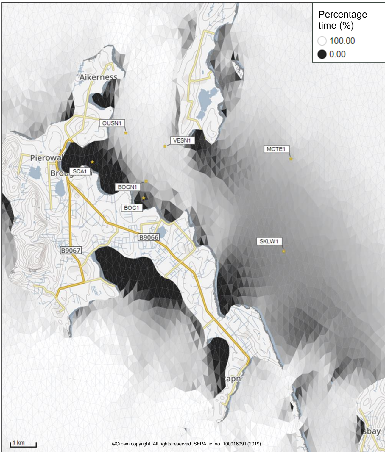
Figure 3: Modelled percentage of time the water flow speed is above 0.095 m/s in the sea area surrounding the proposed site (East of Skelwick Skerry (SKLW1)-).
