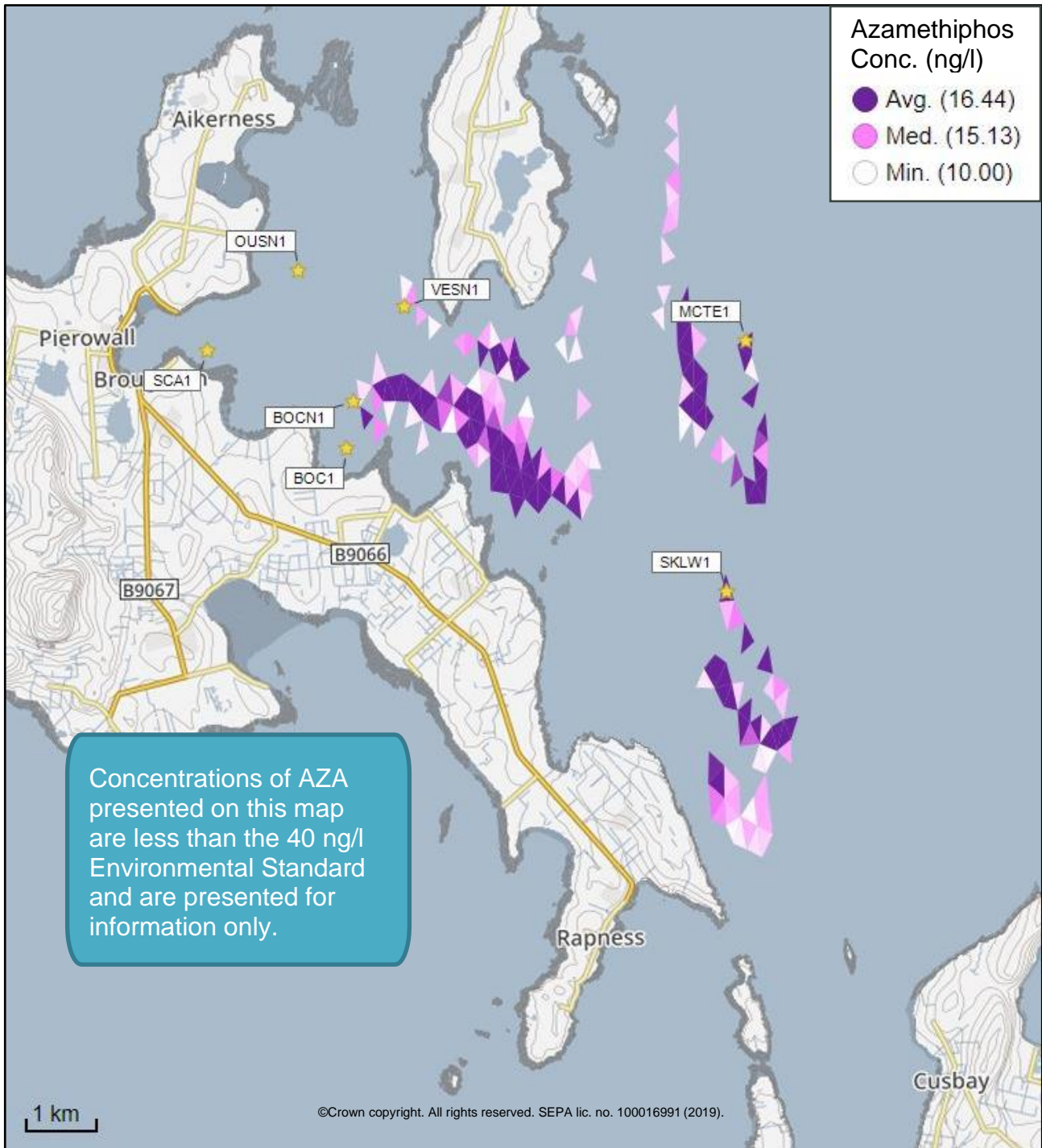
Figure 7: Modelled average Azamethiphos concentration over four days from neap tide release for the proposed site (East of Skelwick Skerry (SKLW1)) and other relevant sites.
