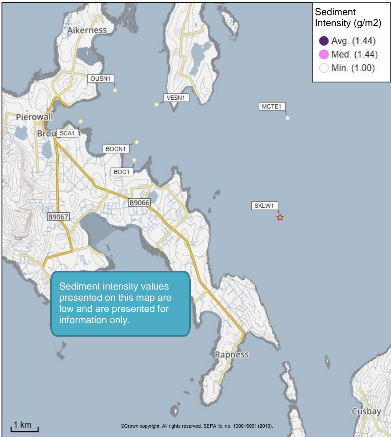
Figure 4: Modelled average sediment intensity over one month for the proposed site only (East of Skelwick Skerry (SKLW1)).
