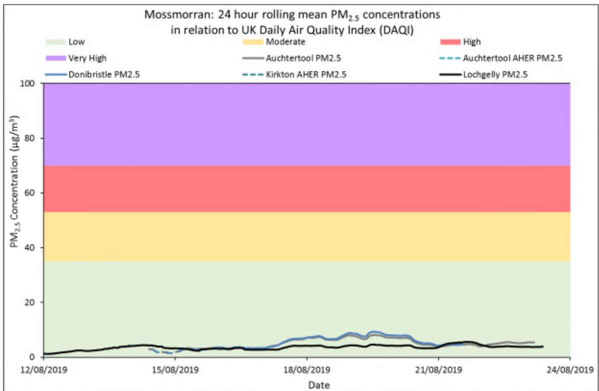
Figure 3: 24 hour rolling means for PM 2.5 at Lochgelly, Auchtartool, Donibristle and the AHER deployments. Line graphs with dotted lines represent mean values based on less than 24 hours of data collection. Some data may be obscured by other line graphs.
