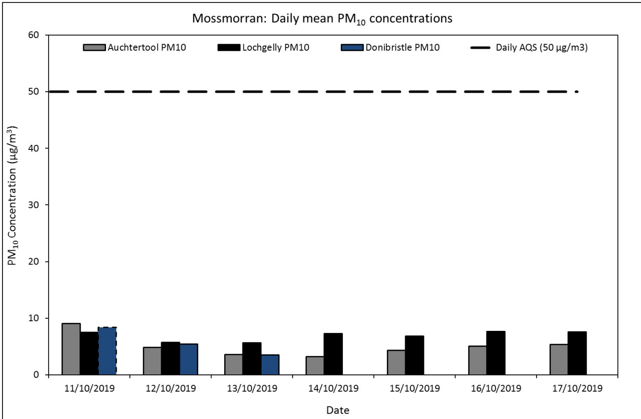
Figure 4: Daily rolling means for PM 10 at Lochgelly, Auchtartool and Donibristle. Dotted lines represent mean values based on less than 24 hours of data collection.
