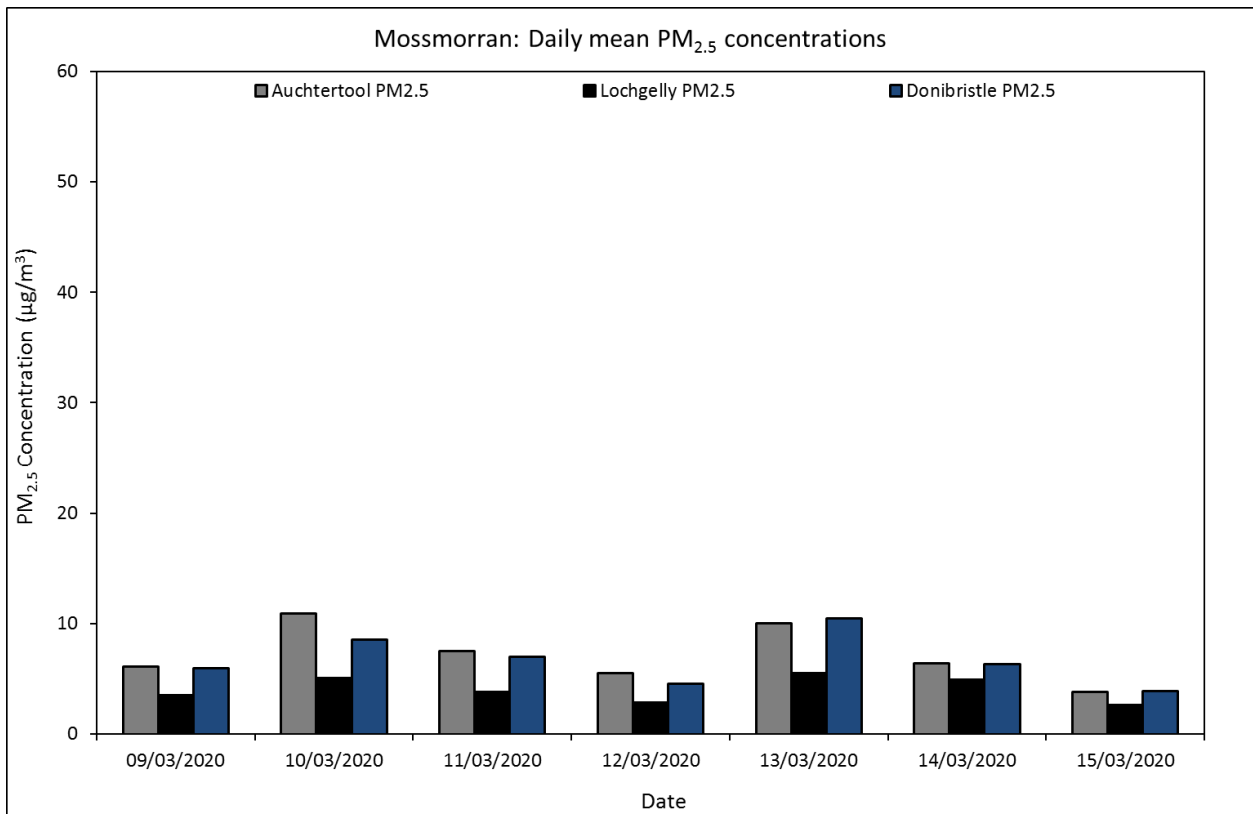
Figure 4: Daily means for PM 2.5 at Lochgelly, Auchtartool and Donibristle. Dotted lines represent mean values based on less than 24 hours of data collection.
