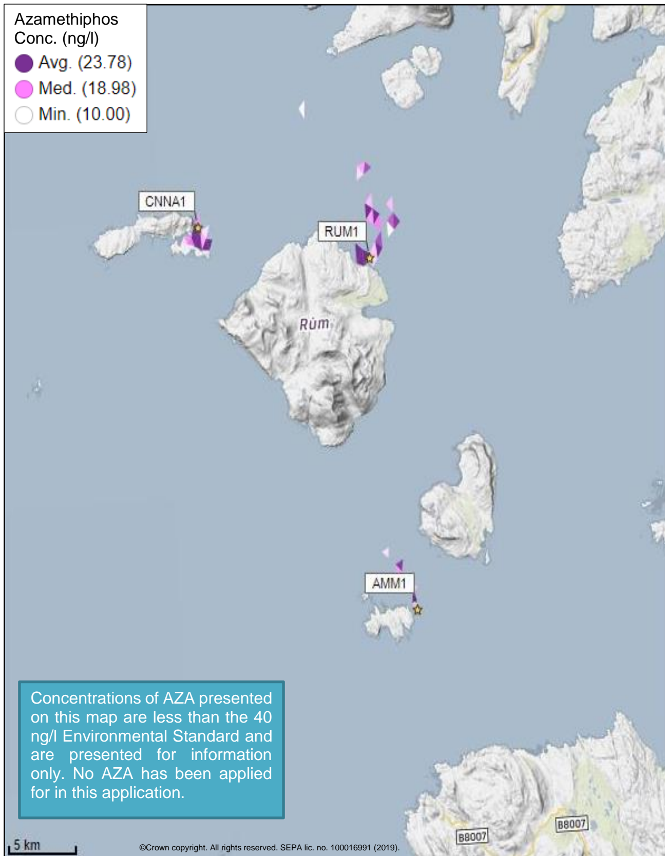
Figure 7: Modelled average Azamethiphos concentration over four days from neap tide release for the proposed site (Canna (CNNA1)) and other relevant sites.
