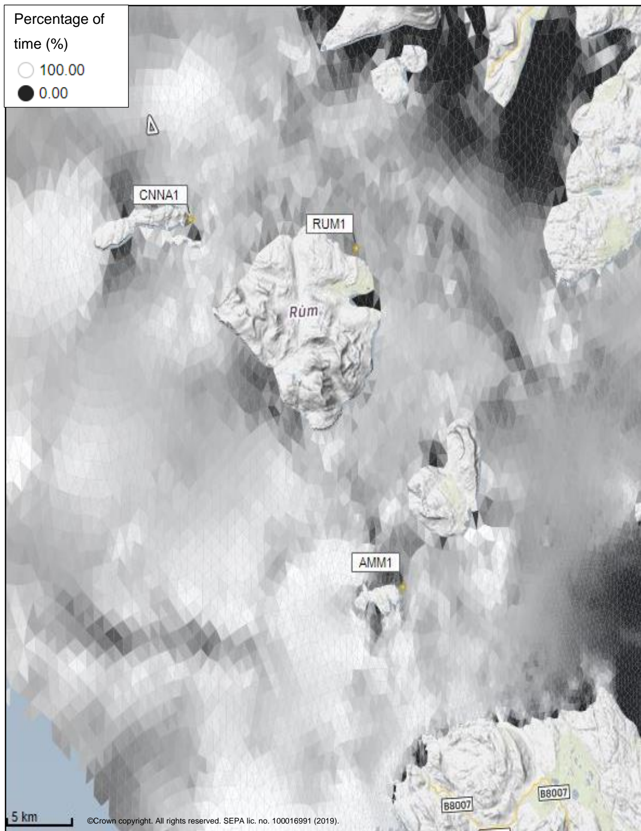
Figure 3: Modelled percentage of time the water flow speed is above 0.095 m/s in the sea area surrounding the proposed site (Canna (CNNA1)).
