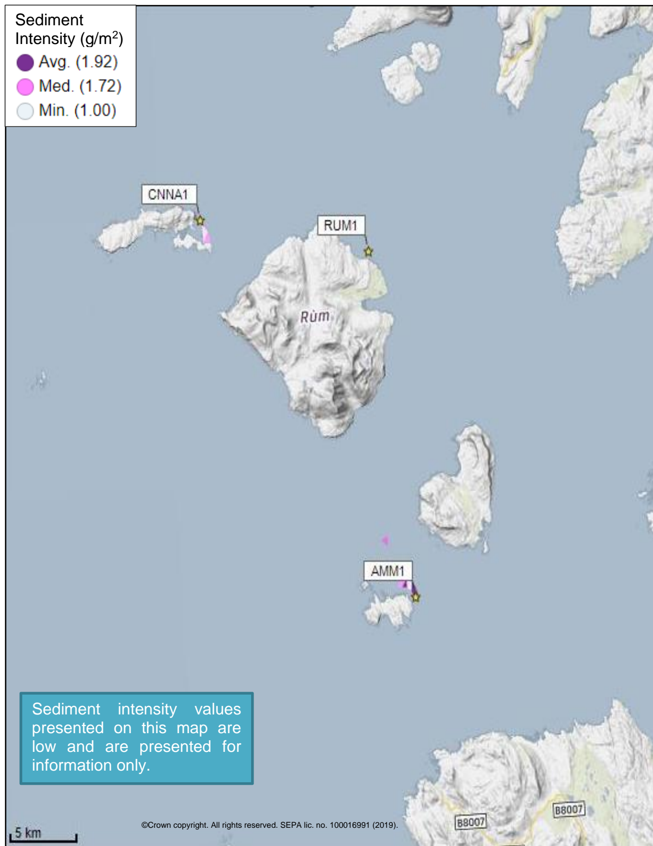
Figure 5: Modelled average sediment intensity over one month for the proposed site (Canna (CNNA1)) and other relevant sites.
