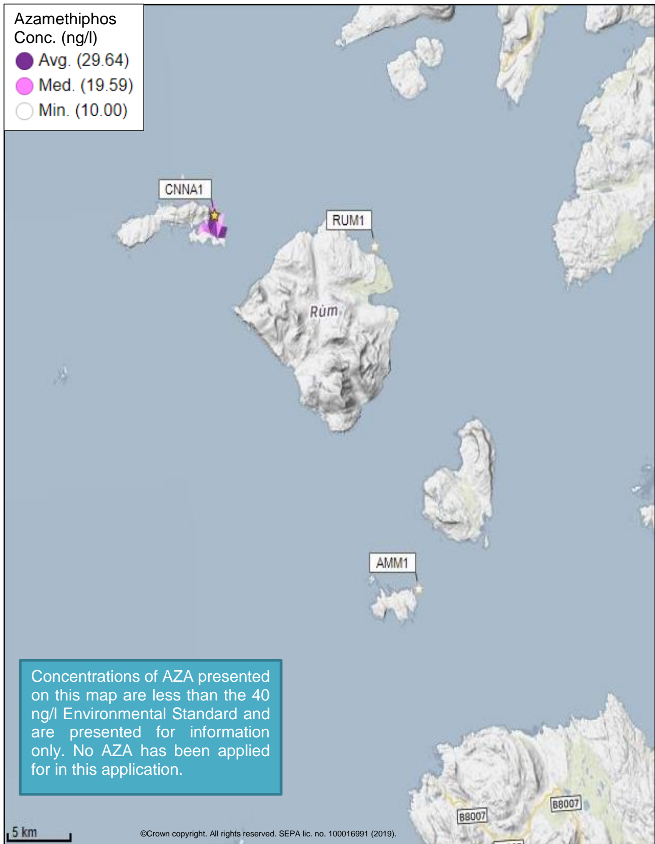
Figure 6: Modelled average Azamethiphos concentration over four days from neap tide release for the proposed site only (Canna (CNNA1)).
