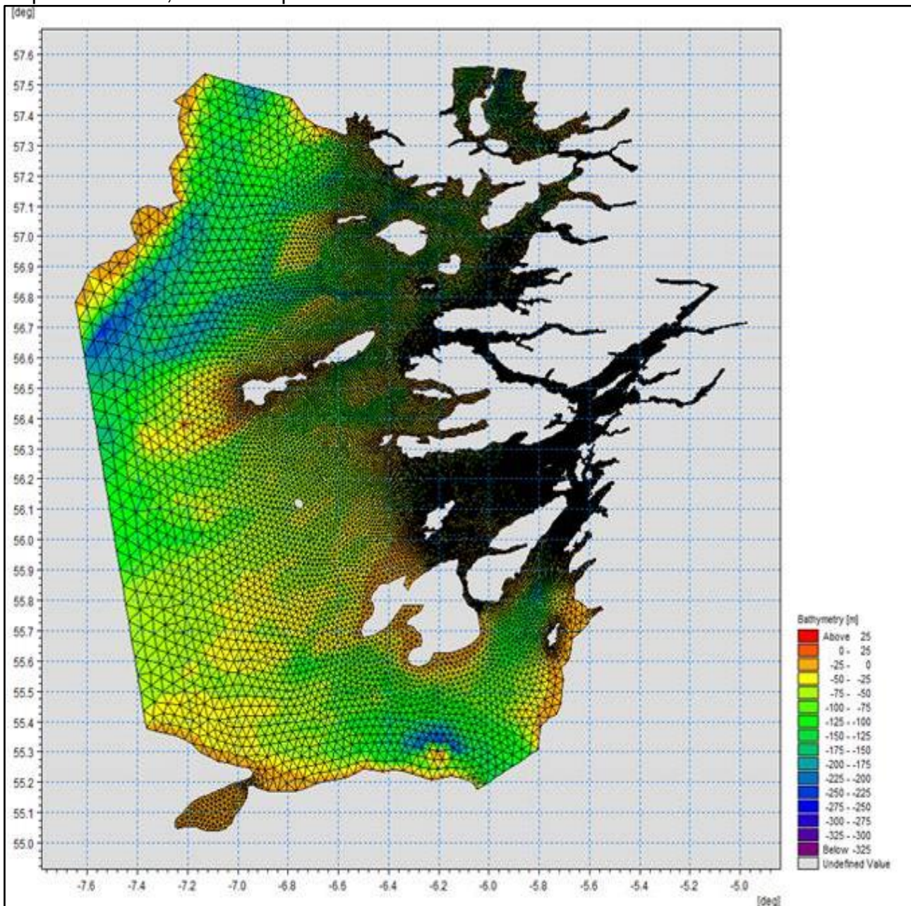
Figure 1: Wider Loch Linnhe System model grid.
