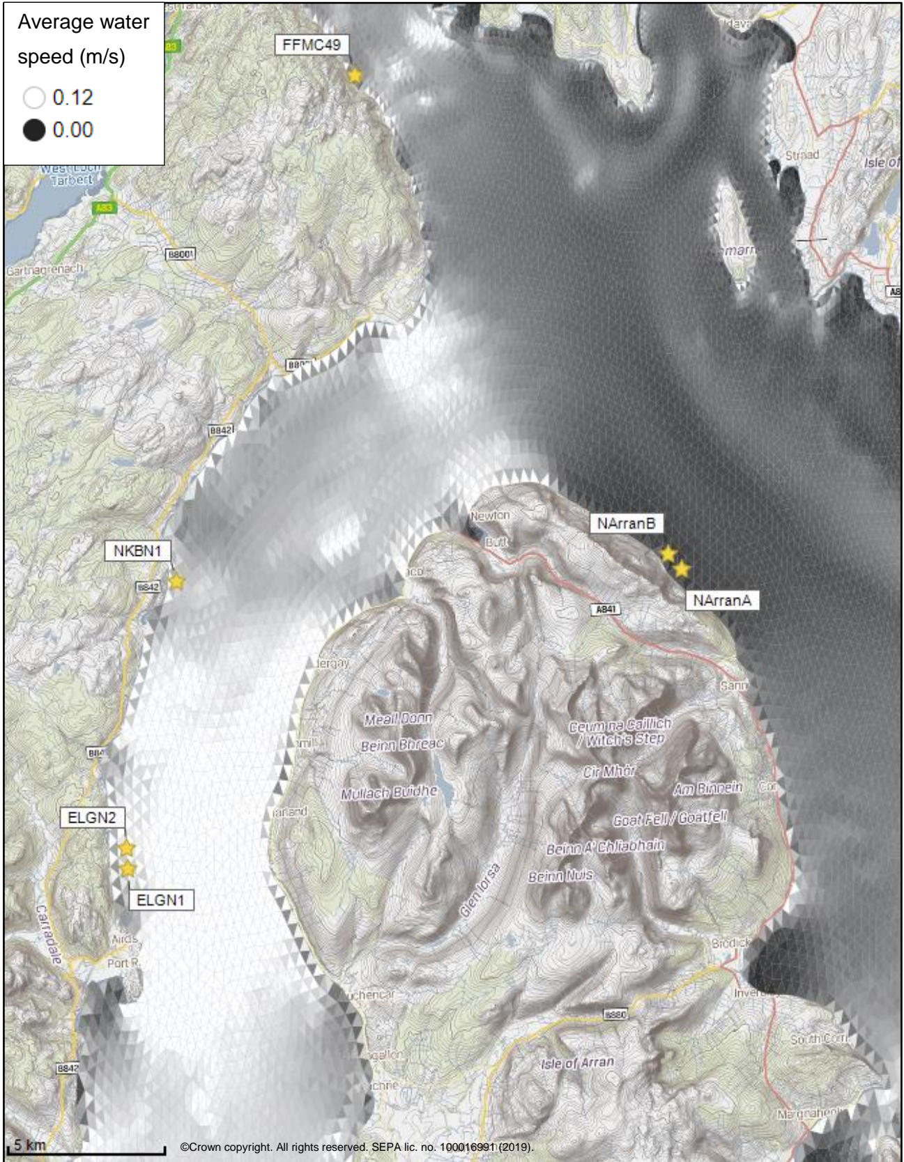
Figure 2: Modelled average water speed (metres per second – m/s) in the sea area surrounding the proposed site (Carradale South (ELGN1)).
