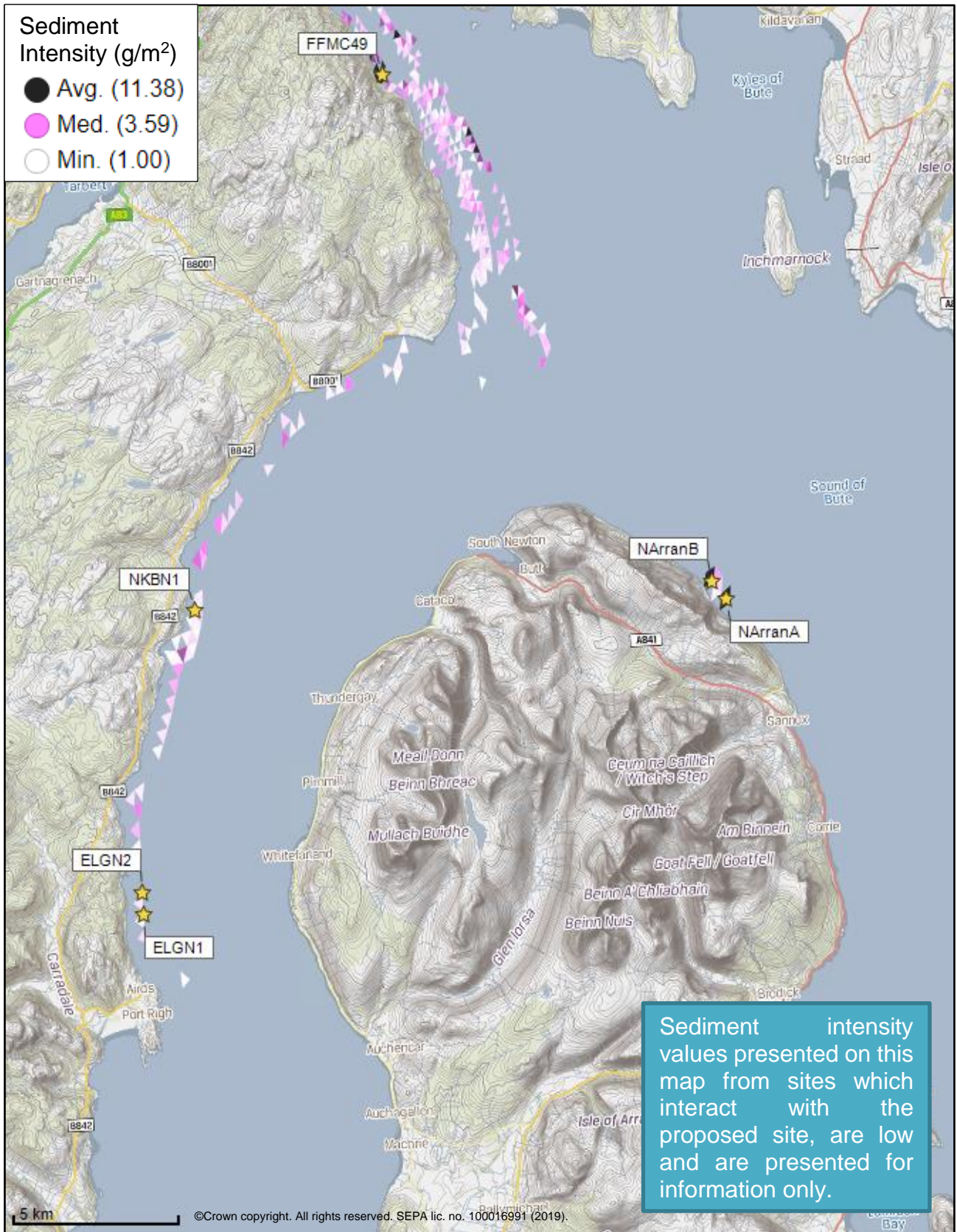
Figure 5: Modelled average sediment intensity over one month for the proposed site (Carradale South (ELGN1)) and other relevant sites.
