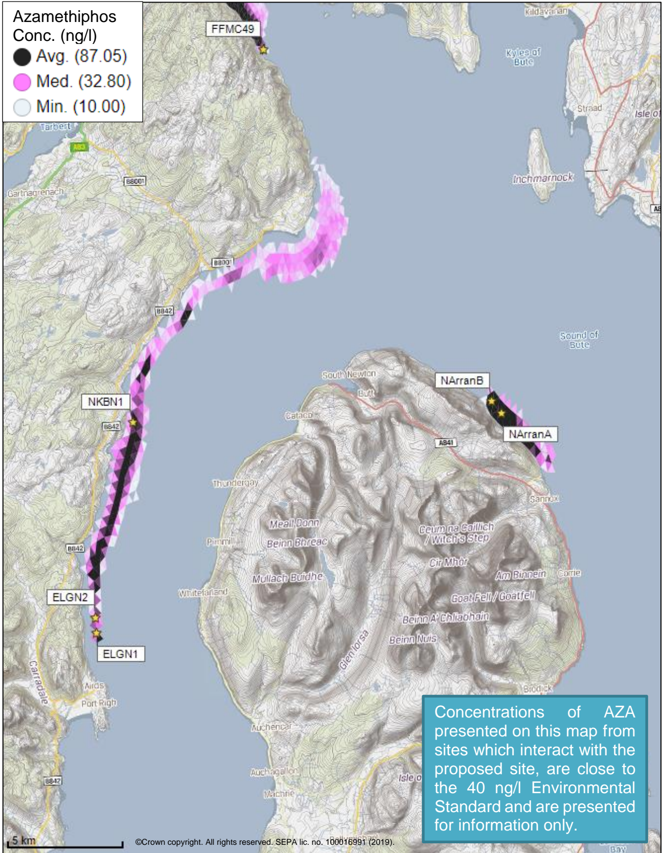
Figure 7: Modelled average Azamethiphos concentration over four days from neap tide release for the proposed site (Carradale South (ELGN1)) and other relevant sites.
