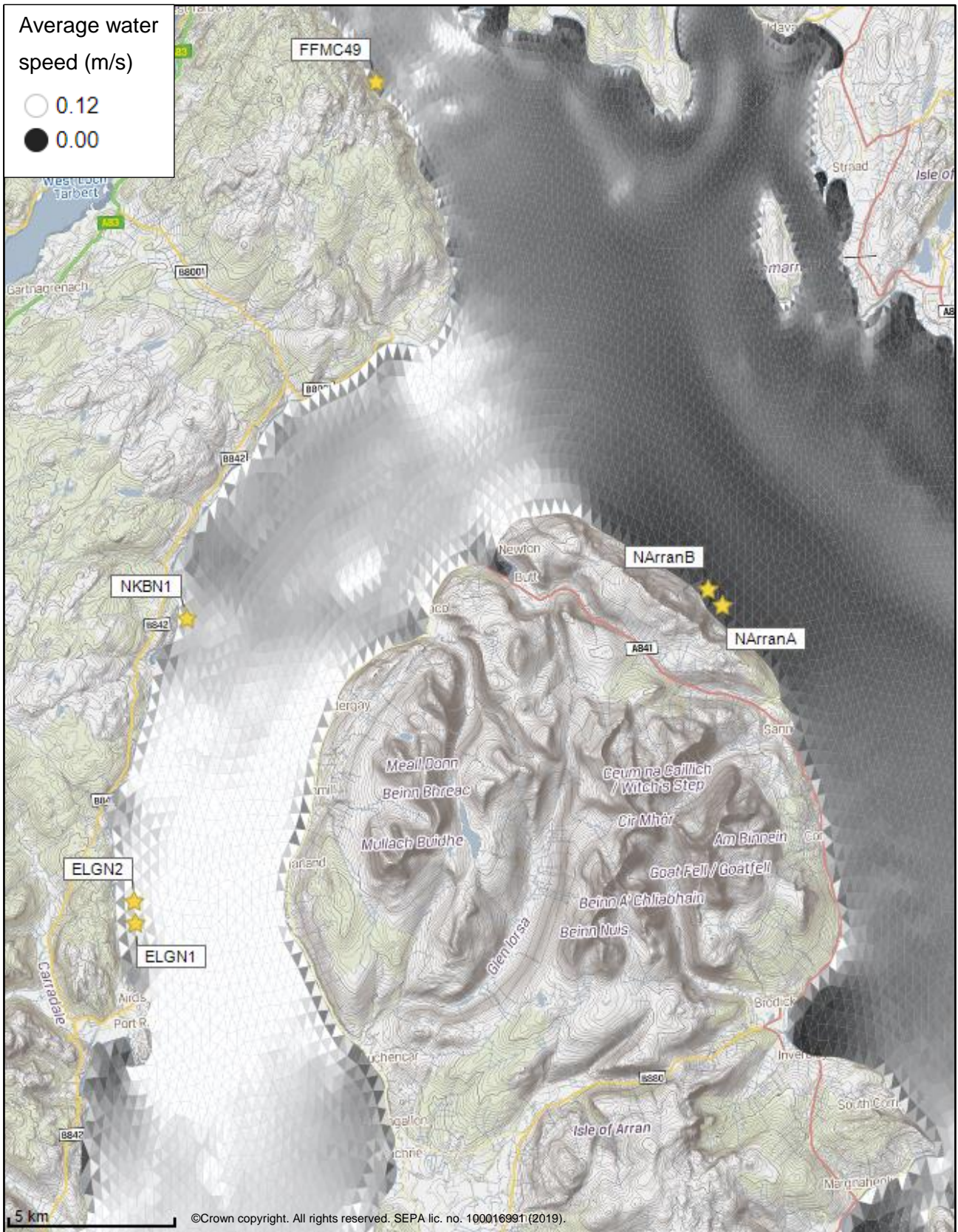
Figure 2: Modelled average water speed (metres per second – m/s) in the sea area surrounding the proposed site (Carradale North (ELGN2)).
