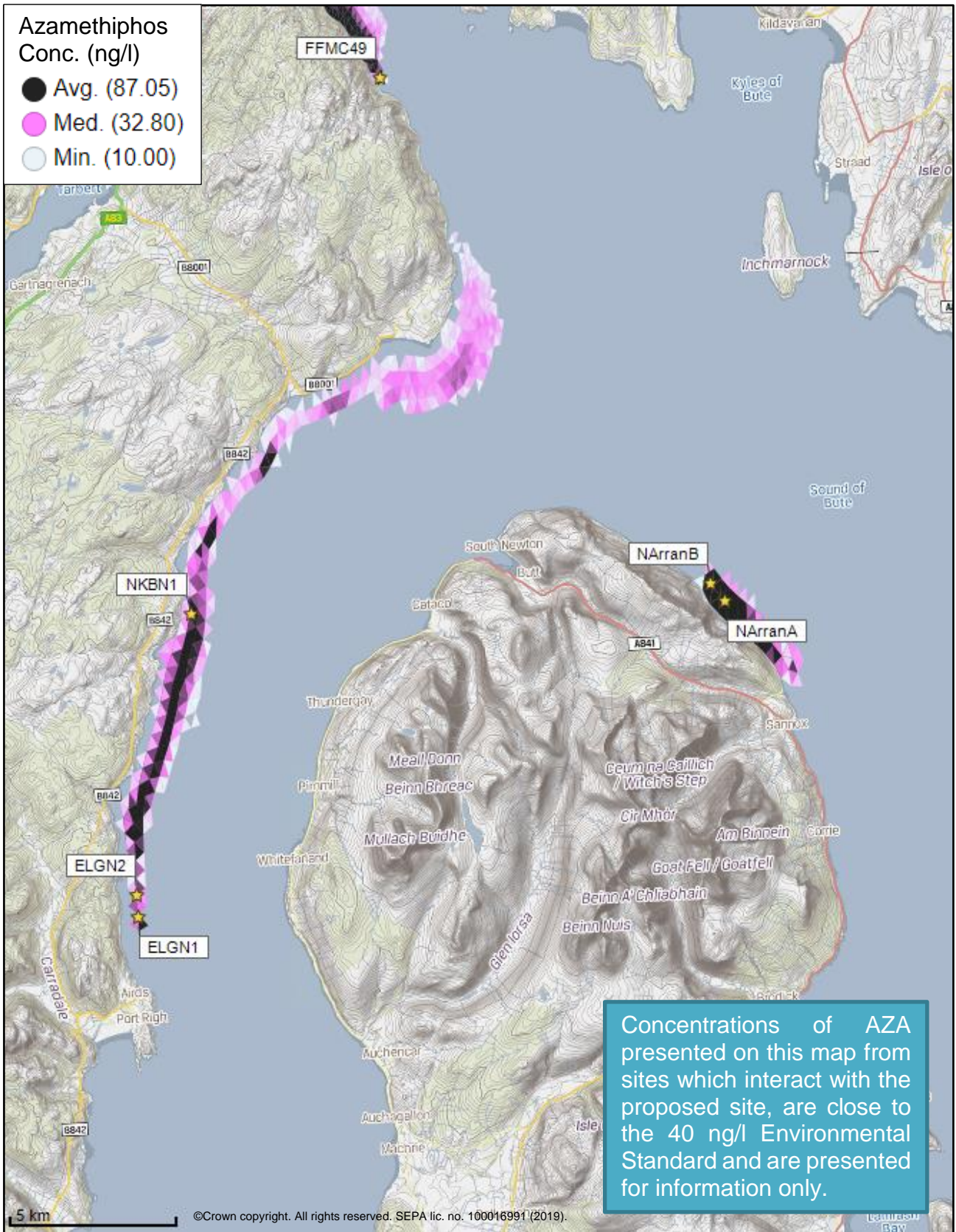
Figure 7: Modelled average Azamethiphos concentration over four days from neap tide release for the proposed site (Carradale North (ELGN2)) and other relevant sites.
