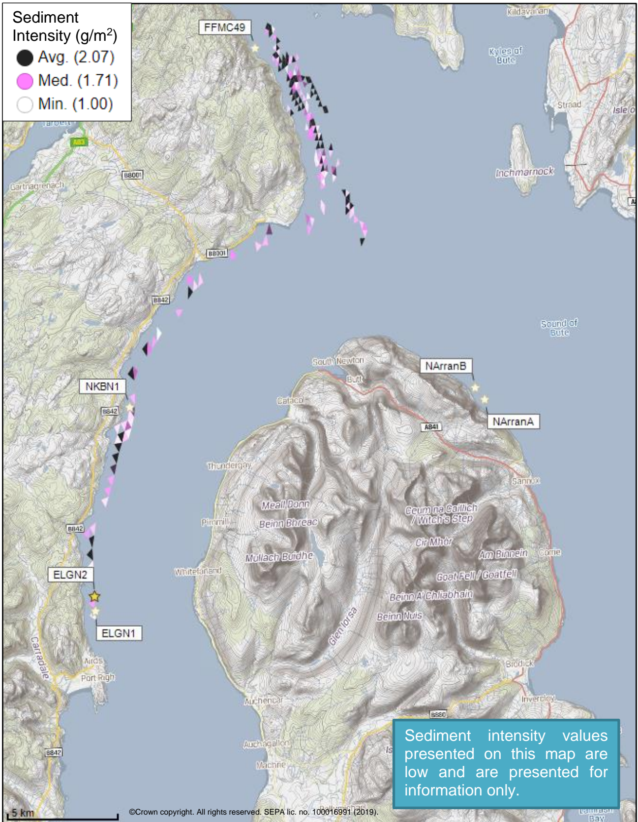
Figure 4: Modelled average sediment intensity over one month for the proposed site only (Carradale North (ELGN2)).
