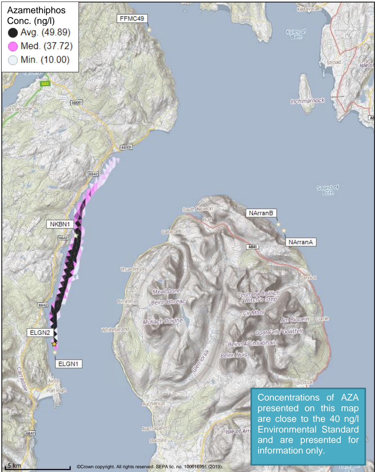
Figure 6: Modelled average Azamethiphos concentration over four days from neap tide release for the proposed site only (Carradale North (ELGN2)).
