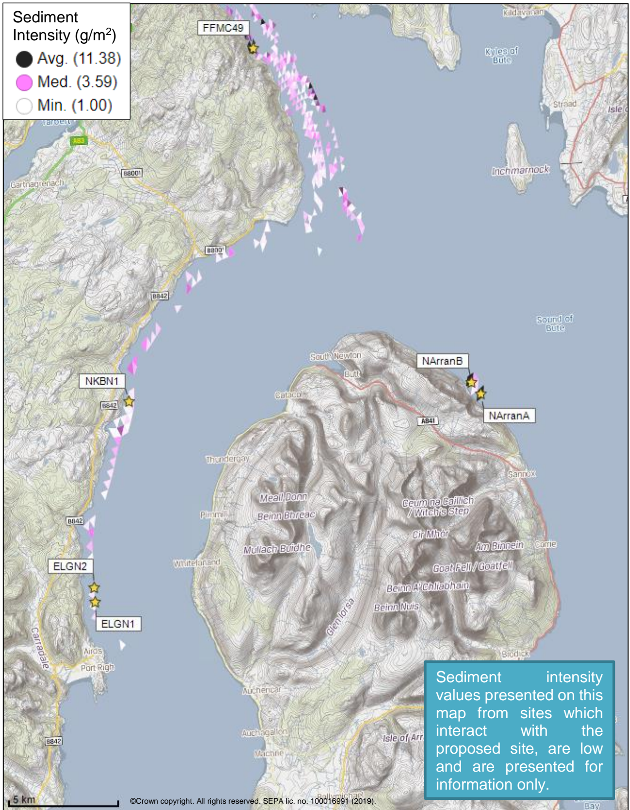
Figure 5: Modelled average sediment intensity over one month for the proposed site (Carradale North (ELGN2)) and other relevant sites.
