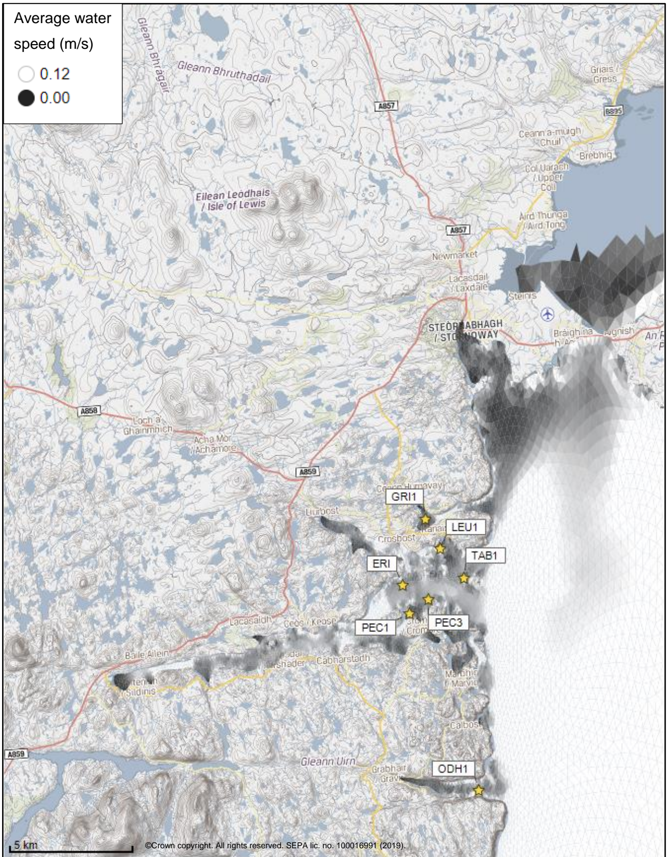
Figure 2: Modelled average water speed (metres per second – m/s) in the sea area surrounding the proposed site (Erisort (ERI)).
