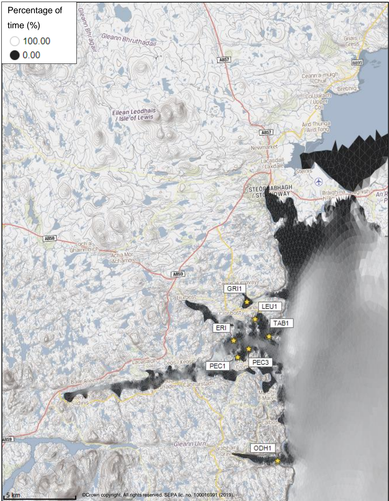
Figure 3: Modelled percentage of time the water flow speed is above 0.095 m/s in the sea area surrounding the proposed site (Erisort (ERI)).
