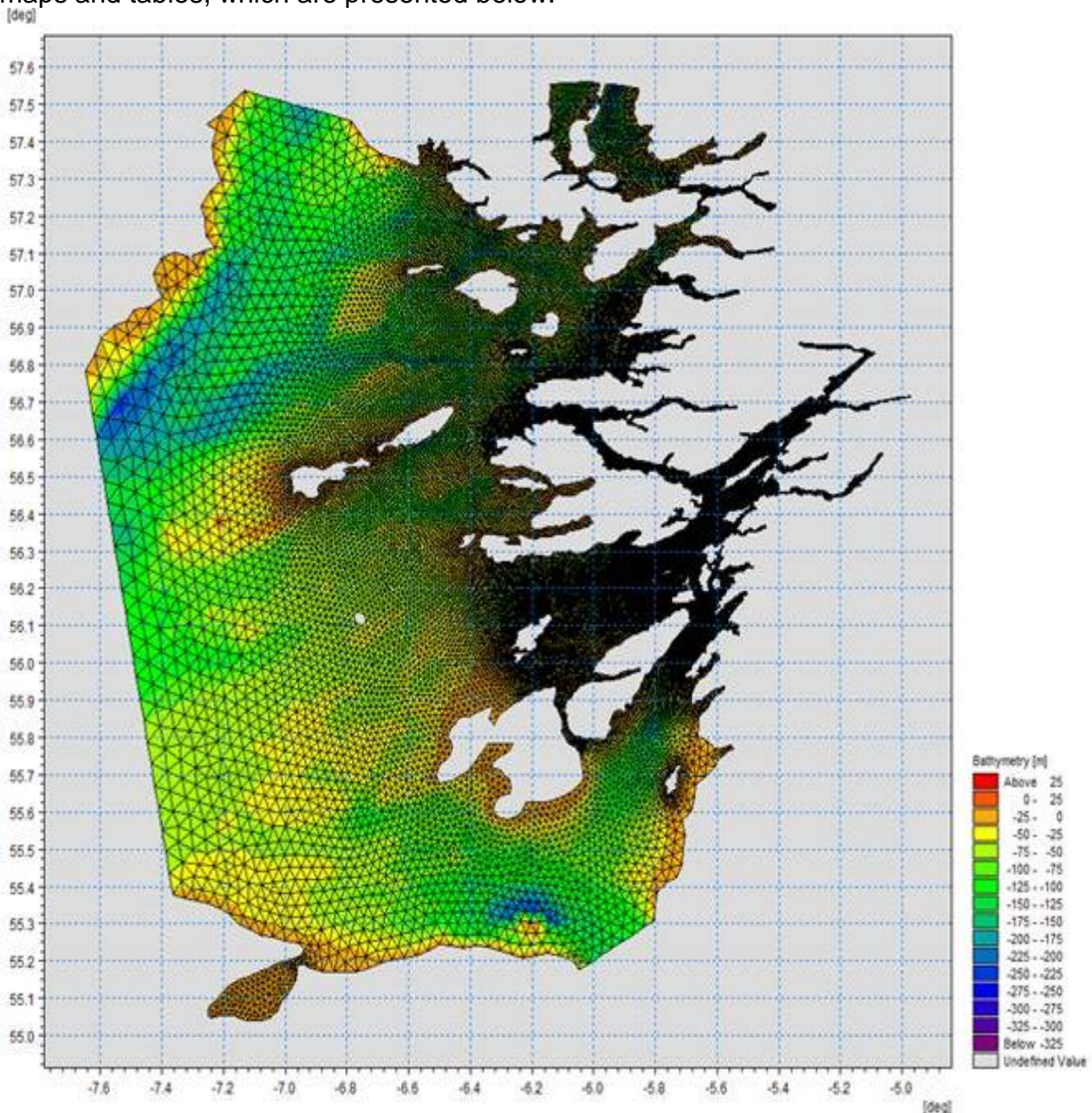
Figure 1: Wider Loch Linnhe System (WLLS) model grid.
