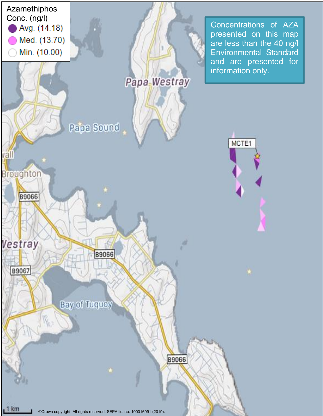
Figure 6: Modelled average Azamethiphos concentration over four days from neap tide release for the proposed site only (East Moclett (MCTE1)).
