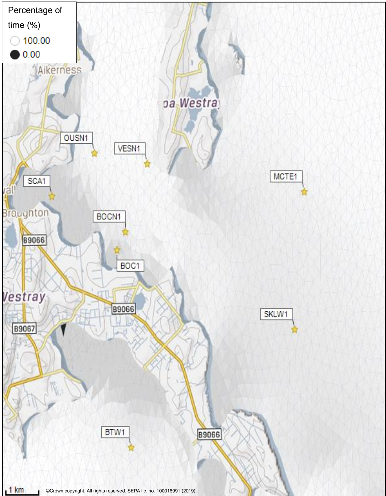
Figure 3: Modelled percentage of time the water flow speed is above 0.095 m/s in the sea area surrounding the proposed site (East Moclett (MCTE1)).
