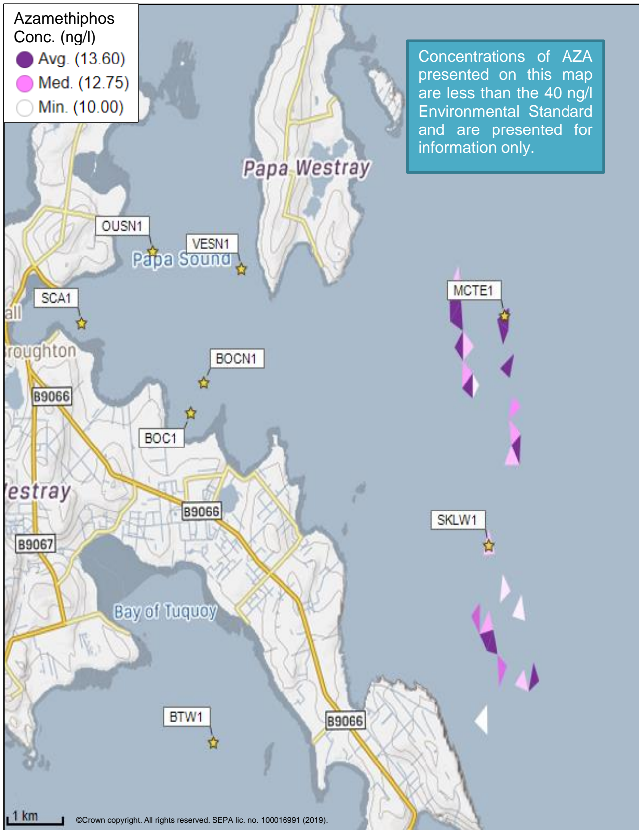
Figure 7: Modelled average Azamethiphos concentration over four days from neap tide release for the proposed site (East Moclett (MCTE1)) and other relevant sites.
