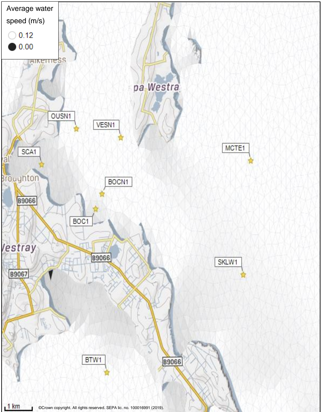
Figure 2: Modelled average water speed (metres per second – m/s) in the sea area surrounding the proposed site (East Moclett (MCTE1)).
