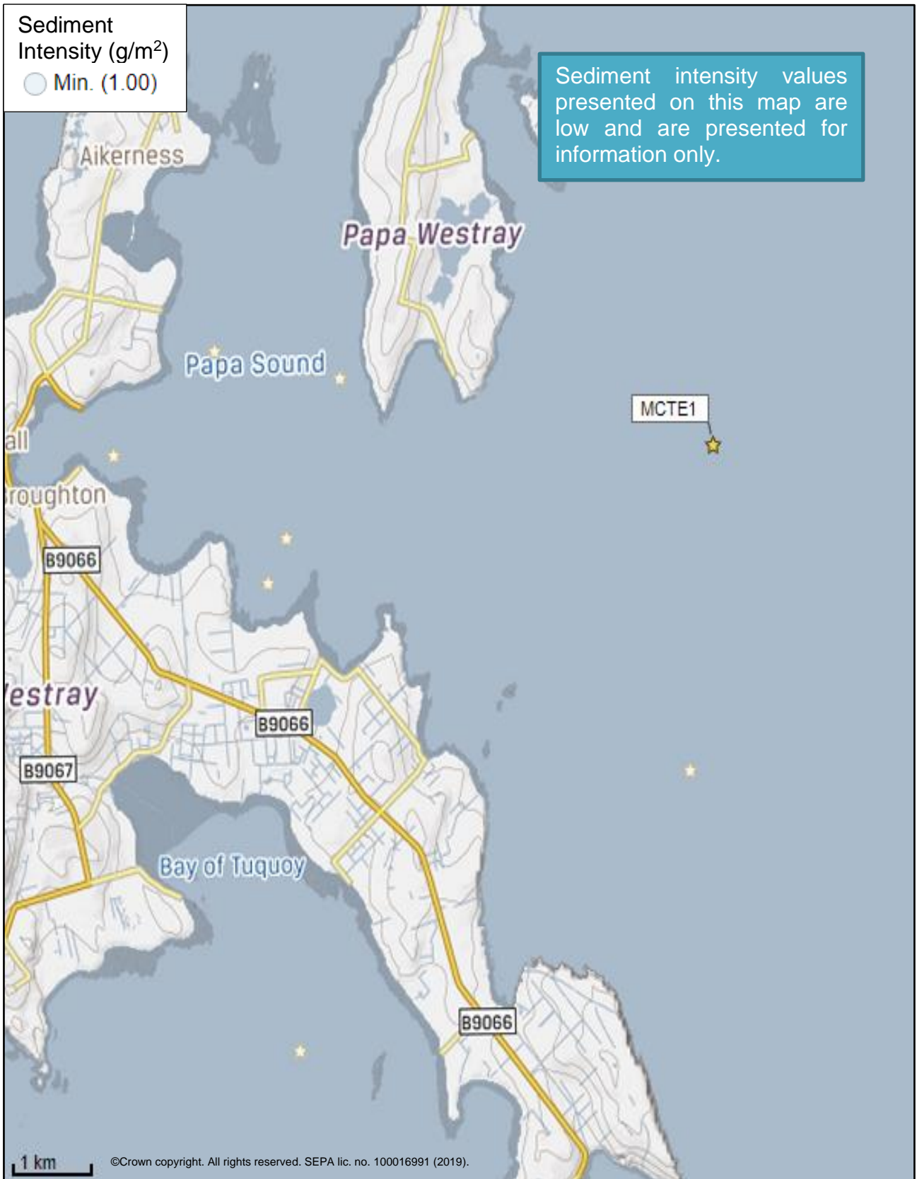
Figure 4: Modelled average sediment intensity over one month for the proposed site only (East Moclett (MCTE1)).
