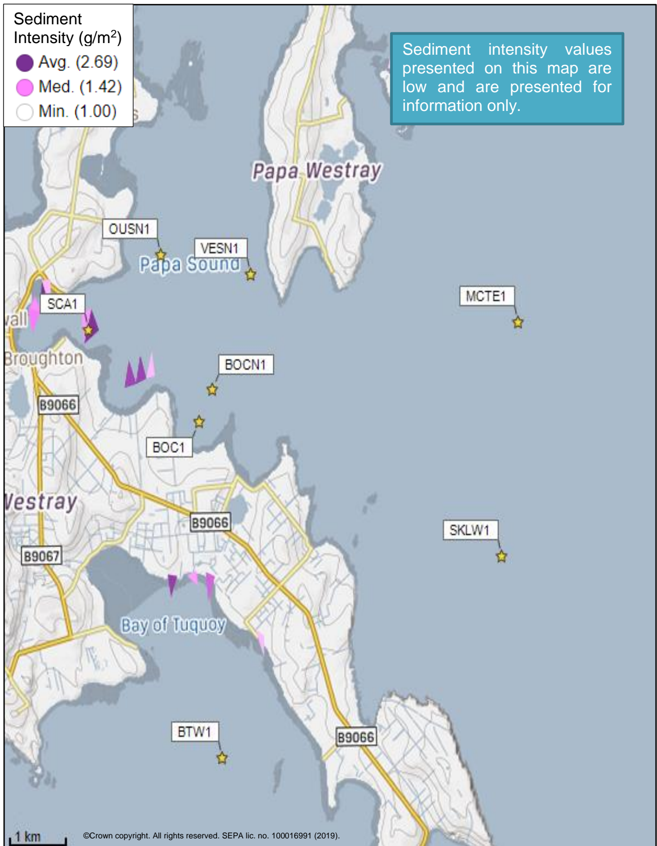
Figure 5: Modelled average sediment intensity over one month for the proposed site (East Moclett (MCTE1)) and other relevant sites.
