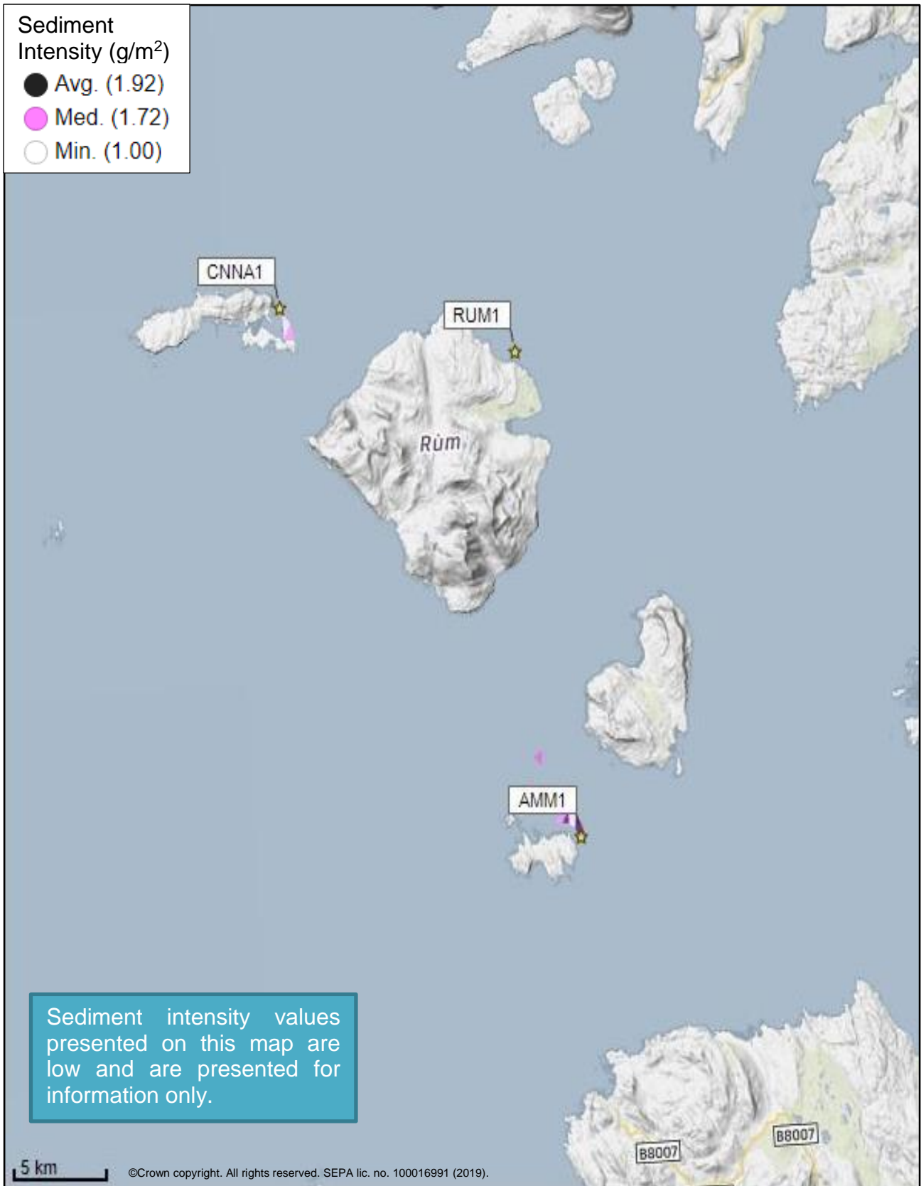
Figure 5: Modelled average sediment intensity over one month for the proposed site (Rum (RUM1)) and other relevant sites.
