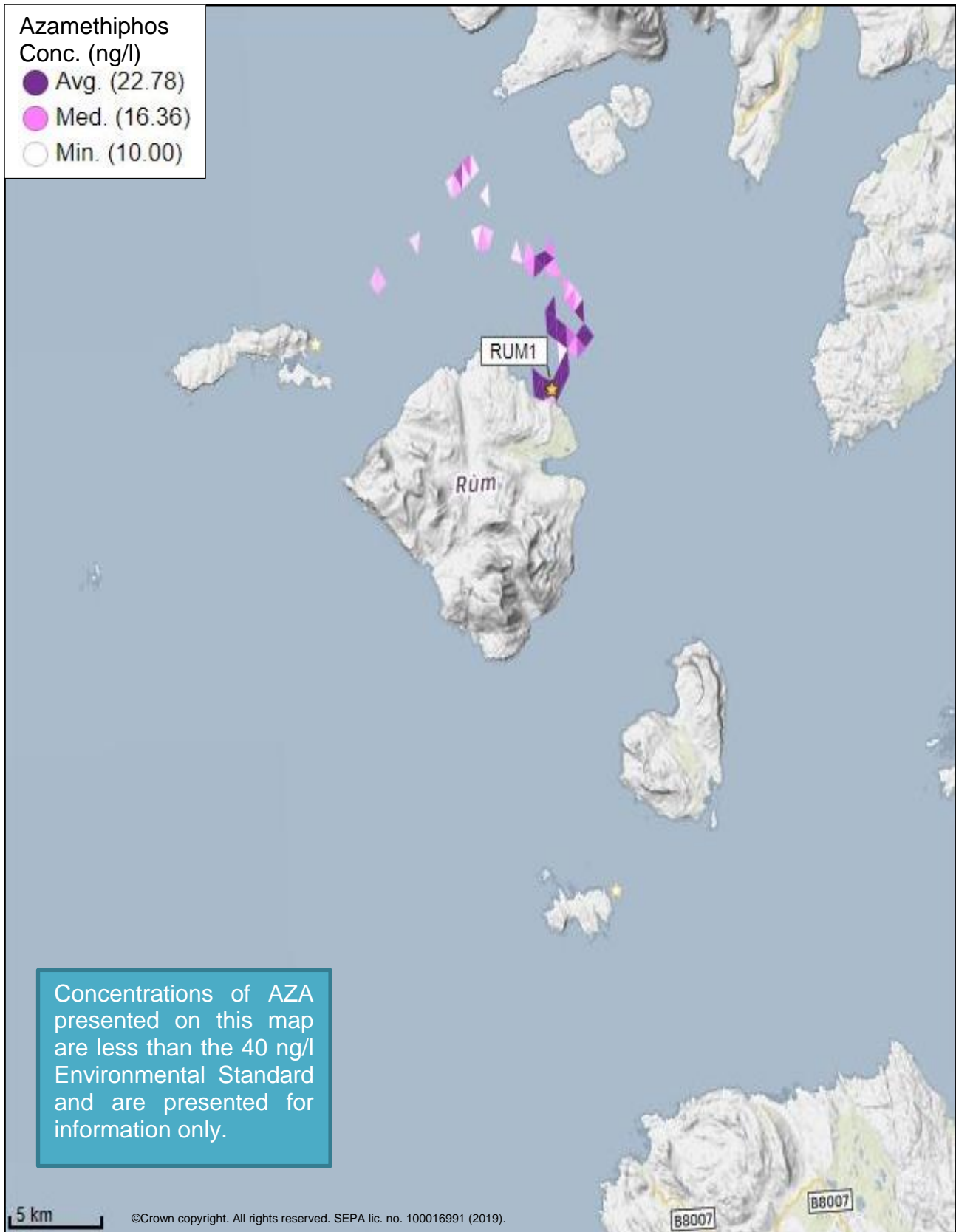
Figure 6: Modelled average Azamethiphos concentration over four days from neap tide release for the proposed site only (Rum (RUM1)).
