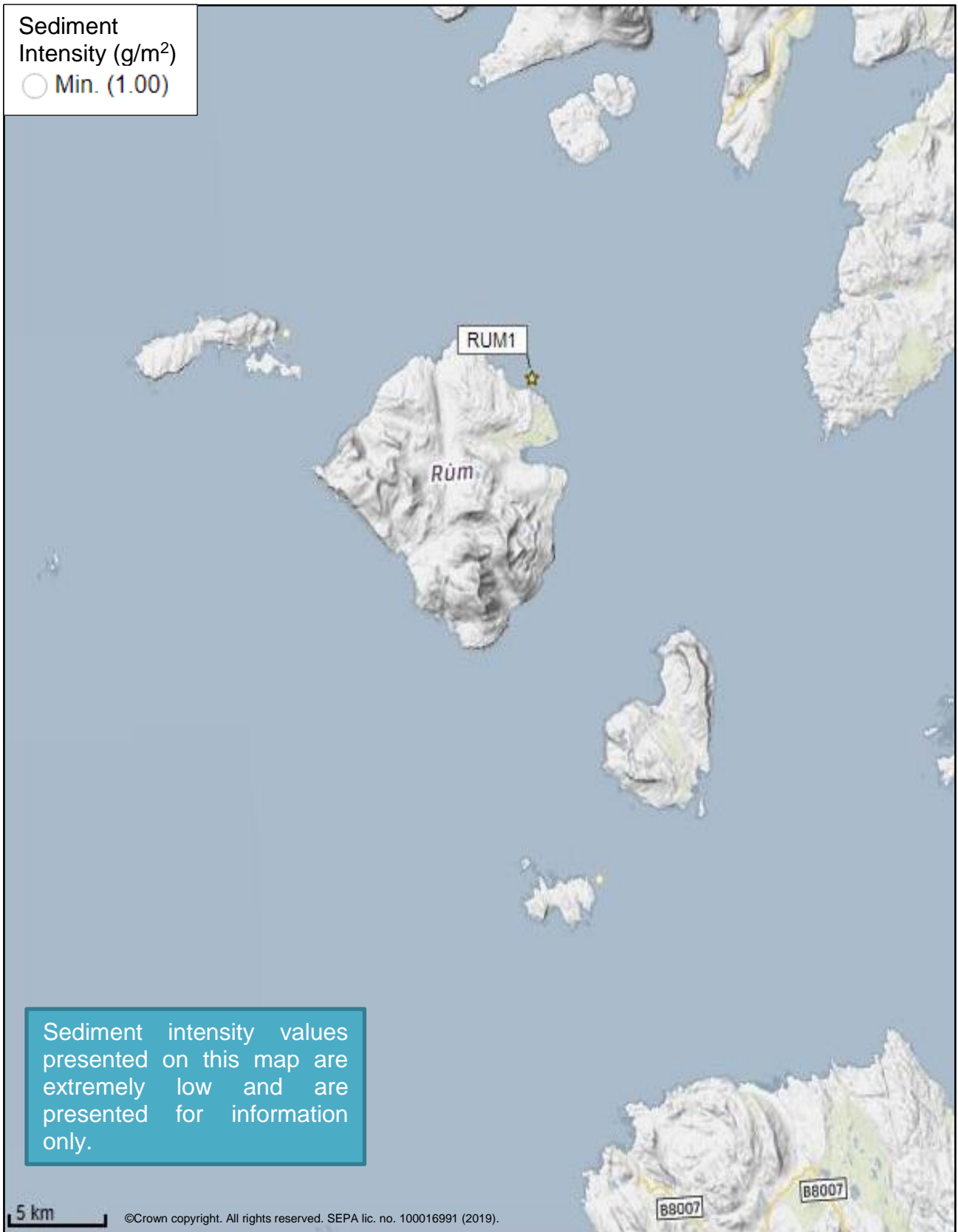
Figure 4: Modelled average sediment intensity over one month for the proposed site only (Rum (RUM1)).
