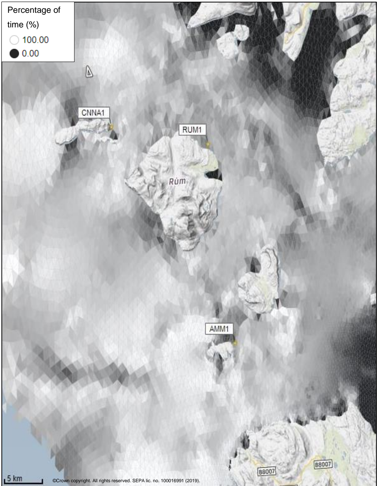
Figure 3: Modelled percentage of time the water flow speed is above 0.095 m/s in the sea area surrounding the proposed site (Rum (RUM1)).
