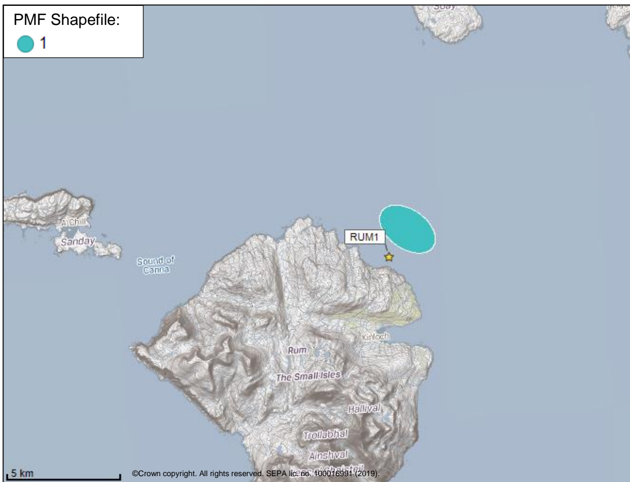
Figure 8. Shapefiles of identified features around the proposed site (Rum (RUM1)).
