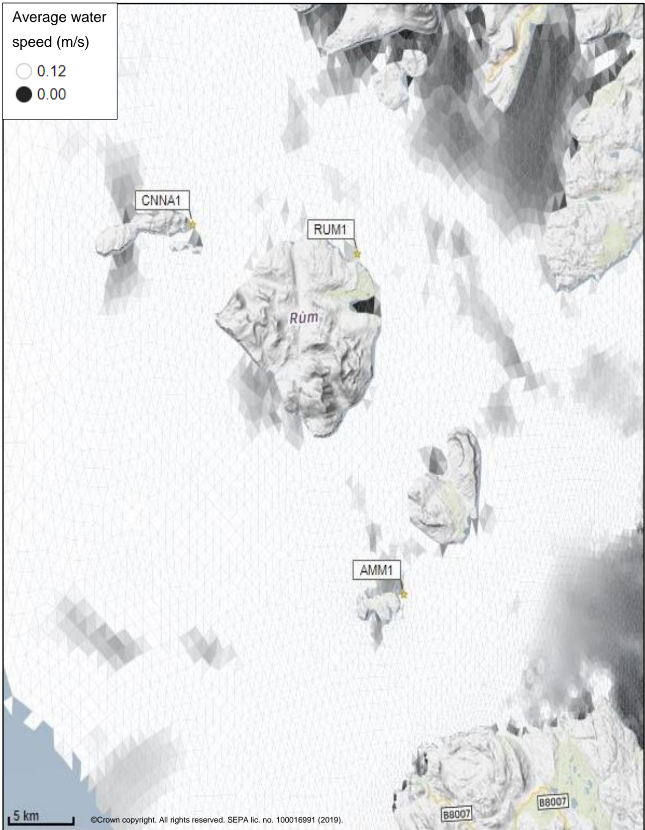
Figure 2: Modelled average water speed (metres per second – m/s) in the sea area surrounding the proposed site (Rum (RUM1)).
