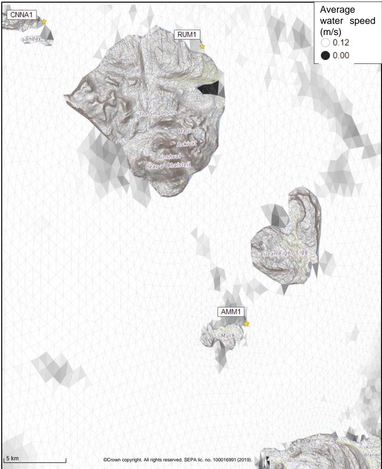
Figure 2: Modelled average water speed (metres per second – m/s) in the sea area surrounding the proposed site (Muck (AMM1)).
