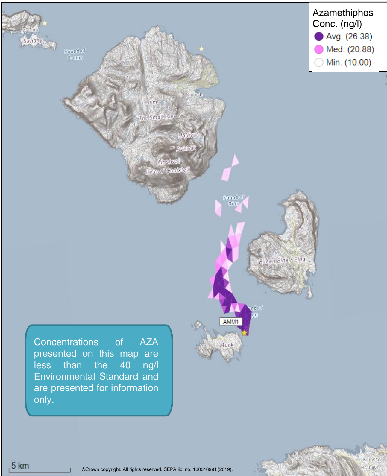
Figure 6: Modelled average Azamethiphos concentration over four days from neap tide release for the proposed site only (Muck (AMM1)).
