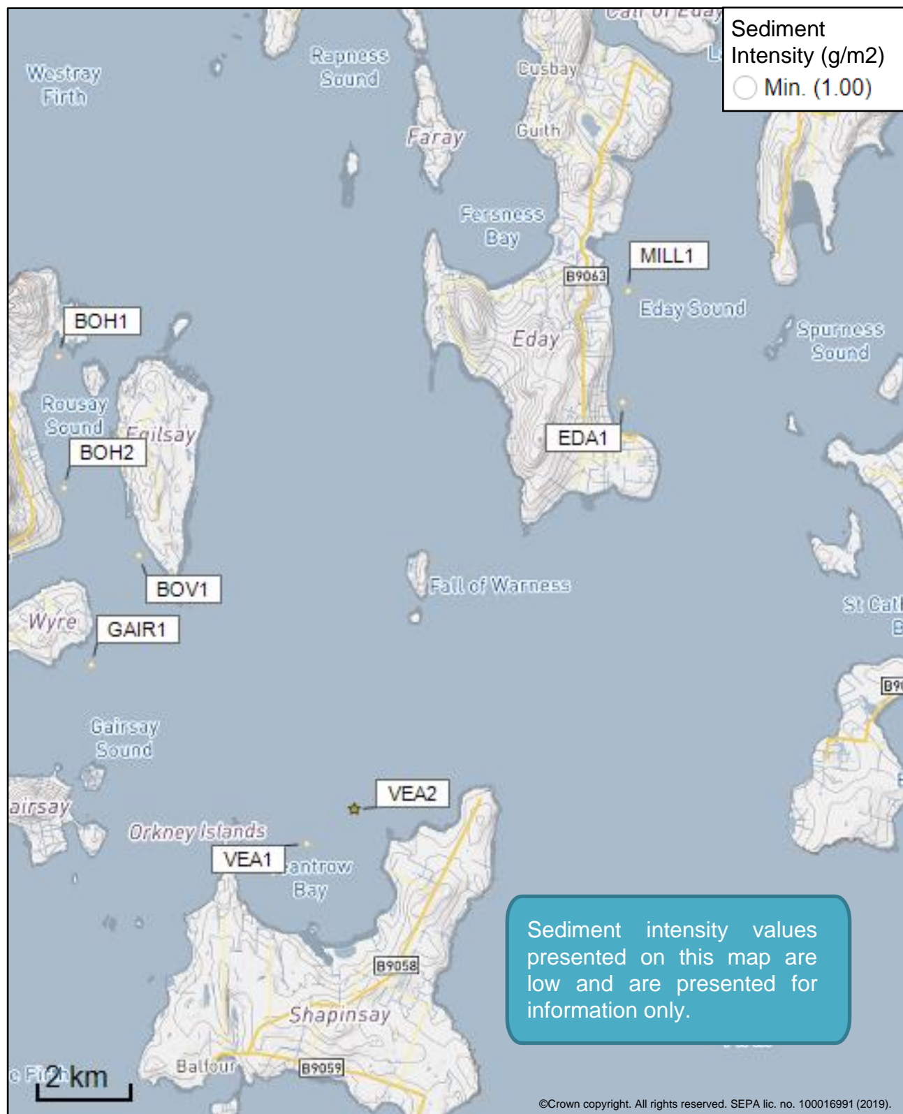
Figure 4: Modelled average sediment intensity over one month for the proposed site only (Shapinsay B (VEA2)).
