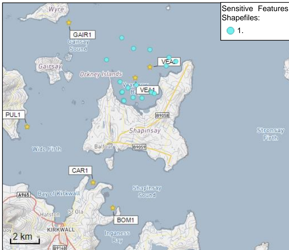
Figure 8. Shapefiles of identified features around the proposed site (Shapinsay B (VEA2)).
