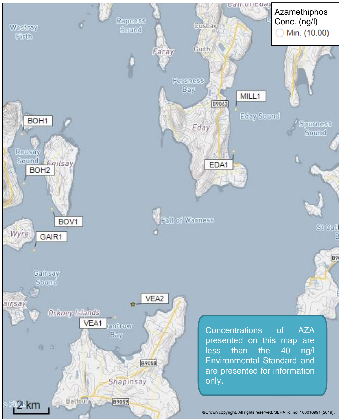
Figure 6: Modelled average Azamethiphos concentration over four days from neap tide release for the proposed site only (Shapinsay B (VEA2)).
