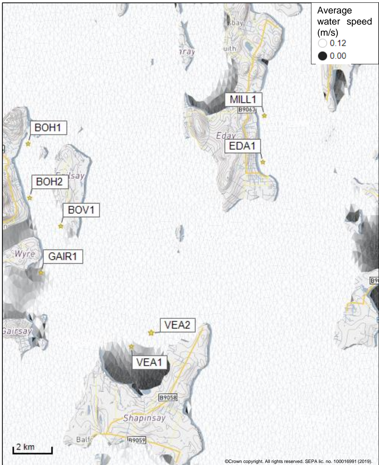
Figure 2: Modelled average water speed (metres per second – m/s) in the sea area surrounding the proposed site (Shapinsay B (VEA2)).
