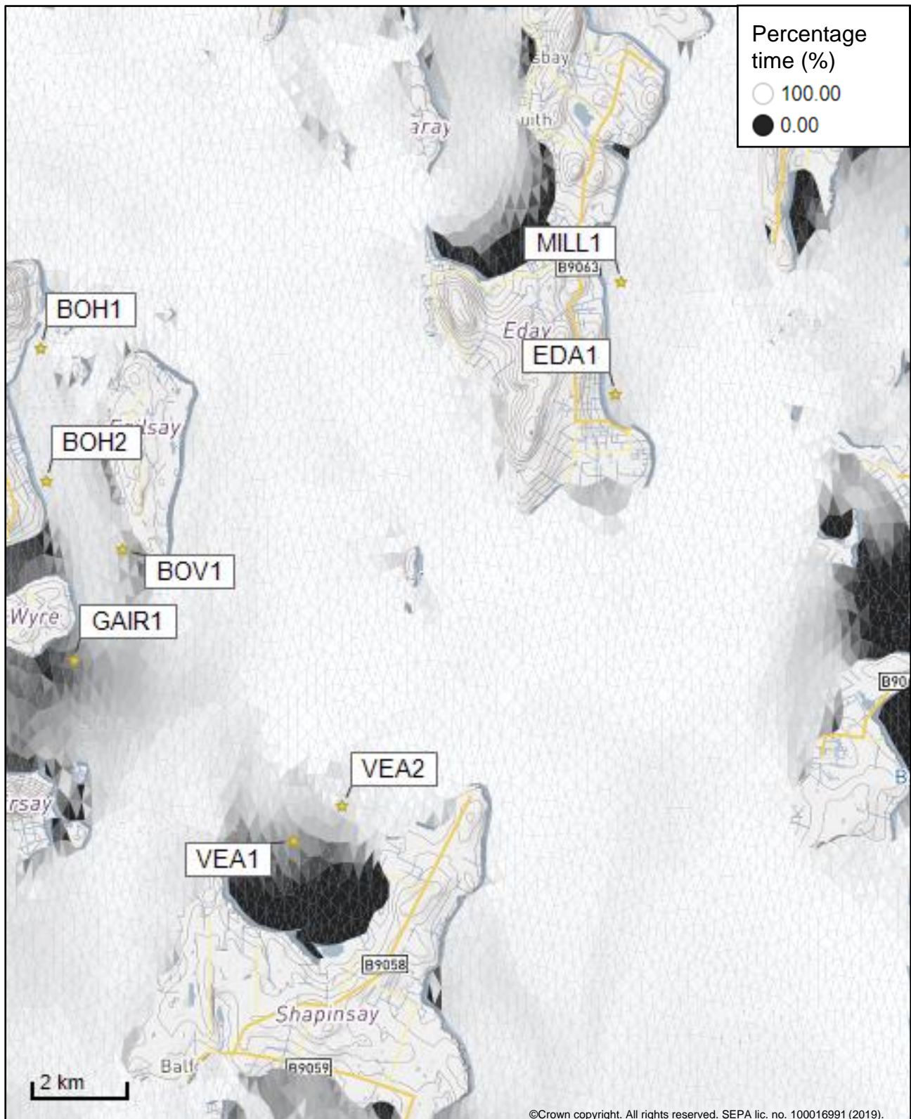
Figure 3: Modelled percentage of time the water flow speed is above 0.095 m/s in the sea area surrounding the proposed site (Shapinsay B (VEA2)).
