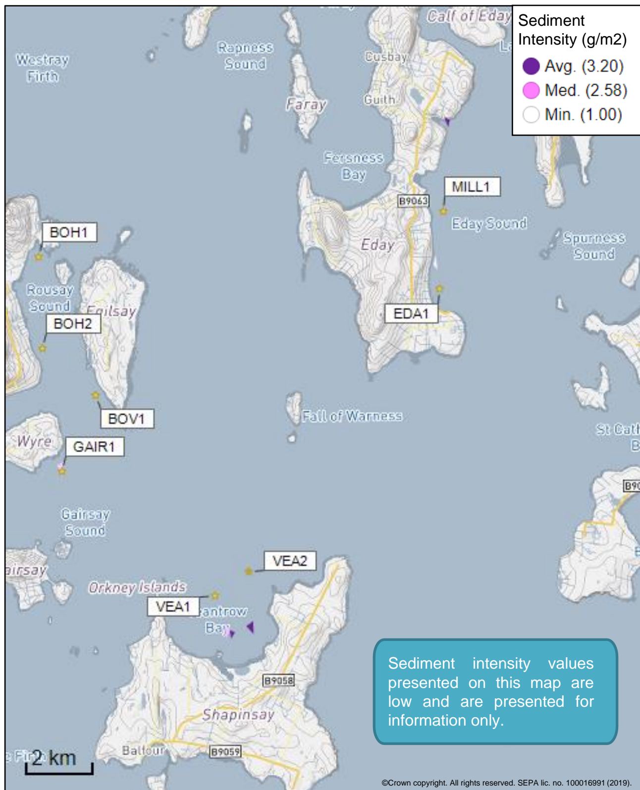
Figure 5: Modelled average sediment intensity over one month for the proposed site (Shapinsay B (VEA2)) and other relevant sites.
