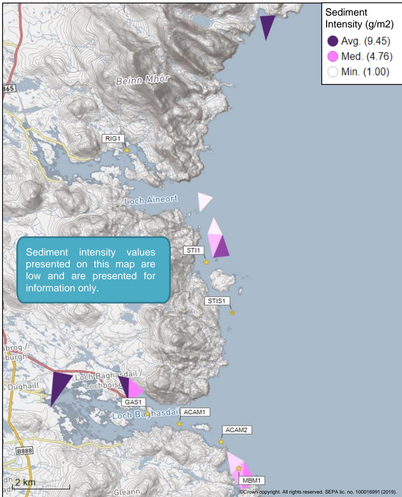
Figure 5: Modelled average sediment intensity over one month for the proposed site (Stulaigh South (STIS1)) and other relevant sites.
