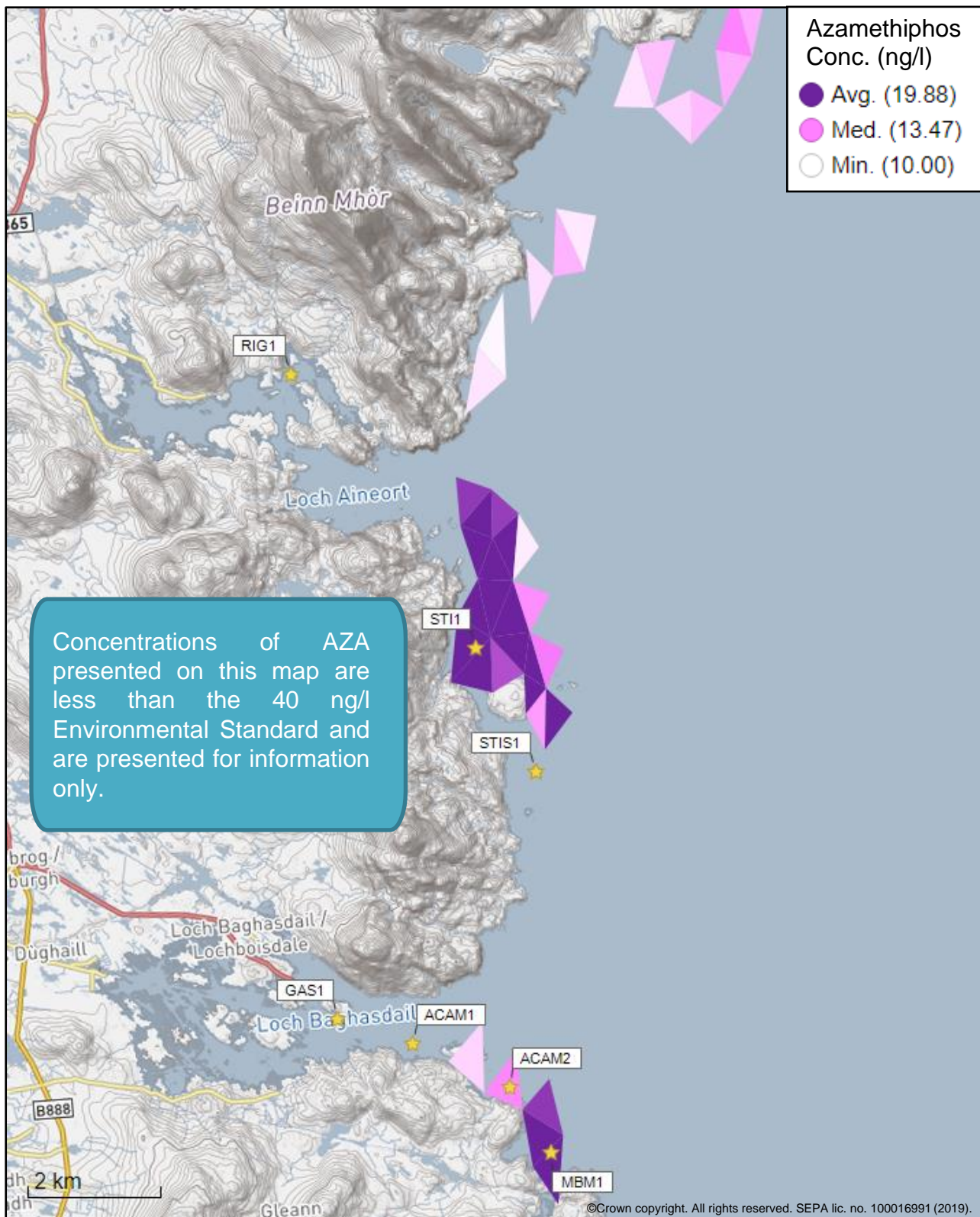
Figure 7: Modelled average Azamethiphos concentration over four days from neap tide release for the proposed site (Stulaigh South (STIS1)) and other relevant sites.
