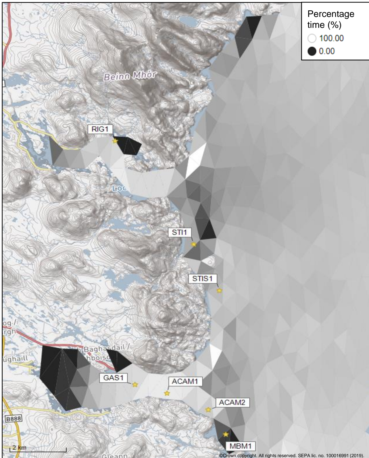
Figure 3: Modelled percentage of time the water flow speed is above 0.095 m/s in the sea area surrounding the proposed site (Stulaigh South (STIS1)).
