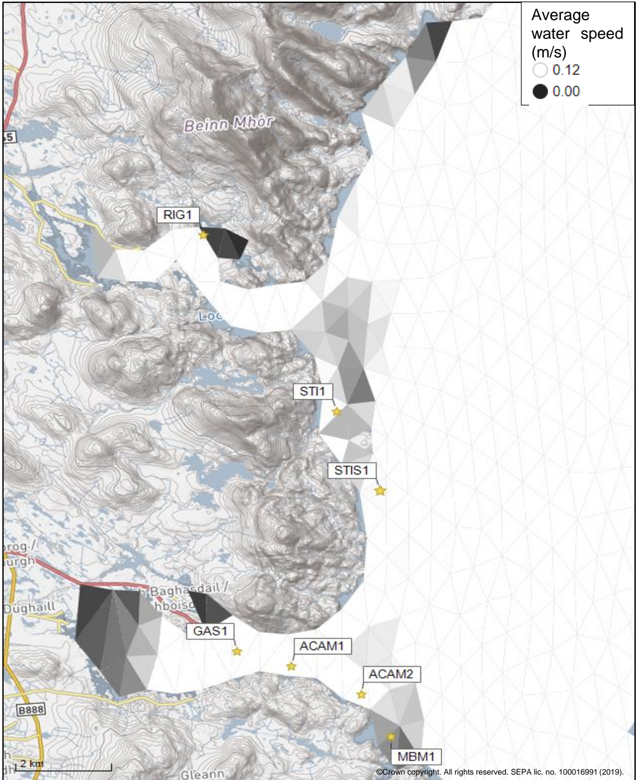
Figure 2: Modelled average water speed (metres per second – m/s) in the sea area surrounding the proposed site (Stulaigh South (STIS1)).
