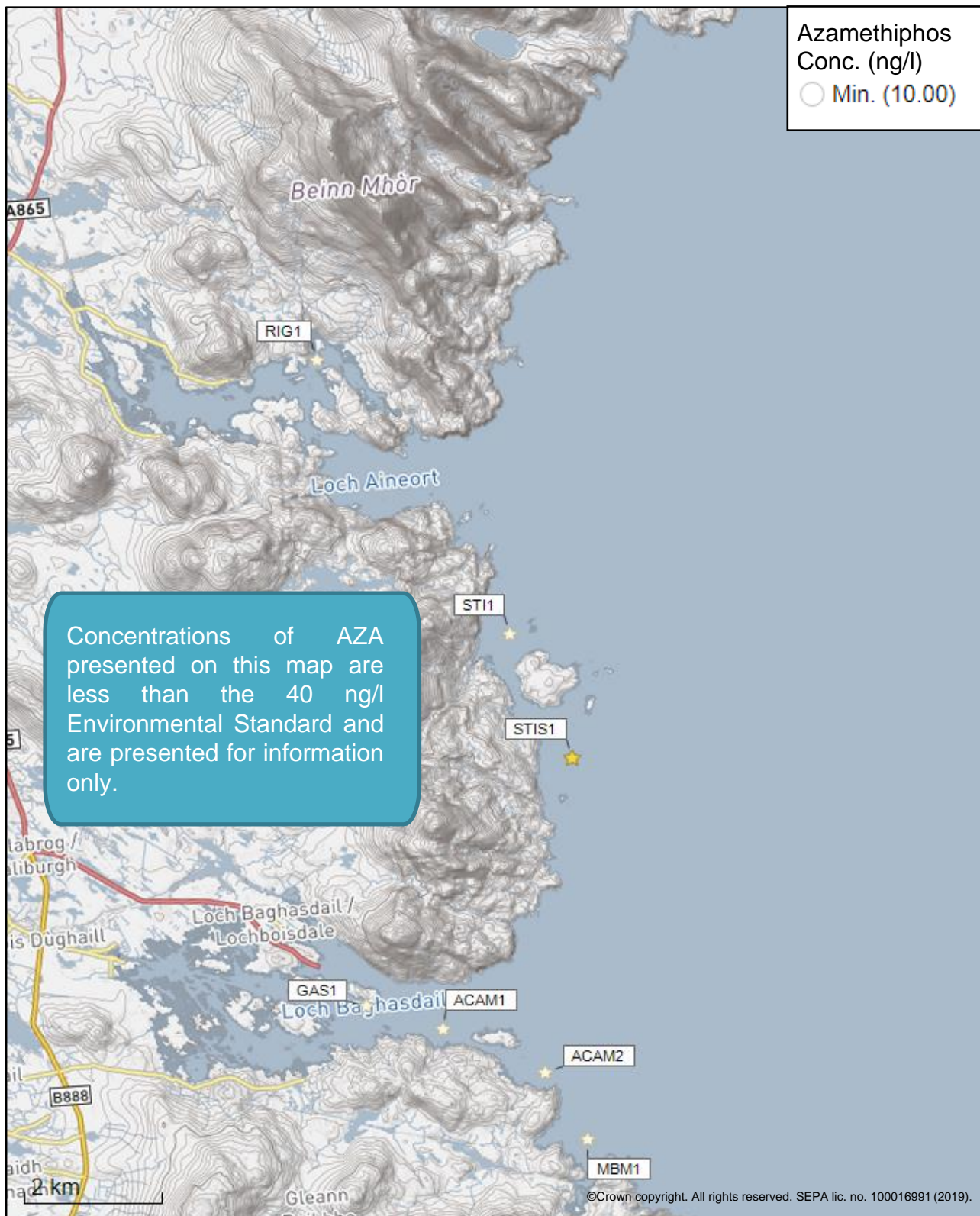
Figure 6: Modelled average Azamethiphos concentration over four days from neap tide release for the proposed site only (Stulaigh South (STIS1)).
