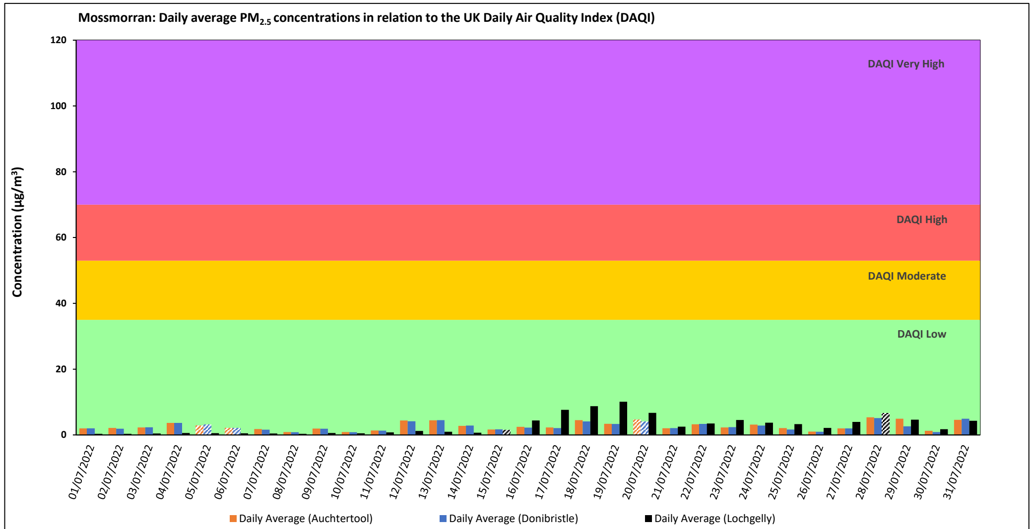
Figure 2: Daily Average PM 2.5 Concentrations at Auchtertool, Donibristle, and Lochgelly: 01-31 July 2022:
