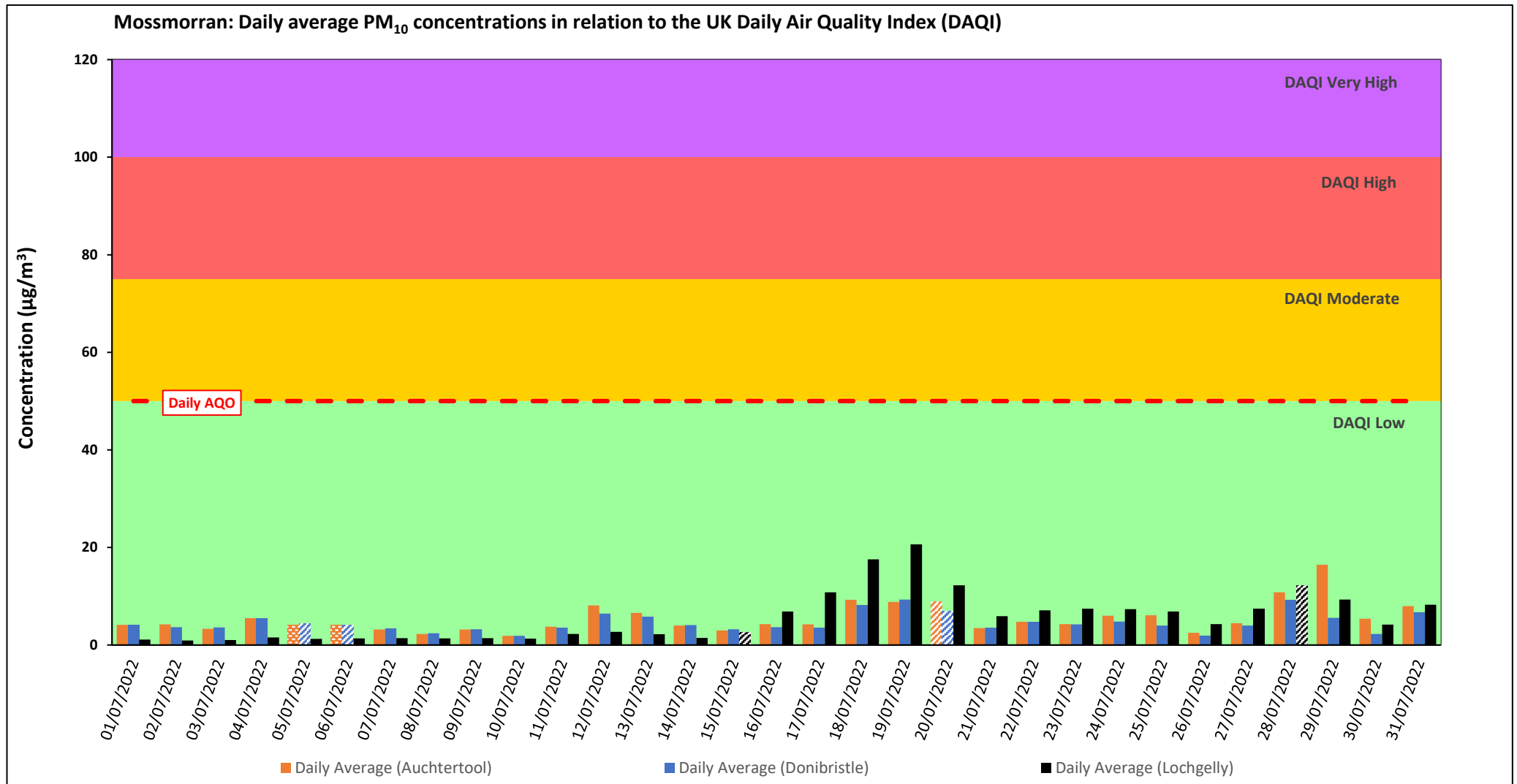
Figure 1: Daily average PM 10 concentrations at Auchtertool, Donibristle and Lochgelly: 01-31 July 2022:
