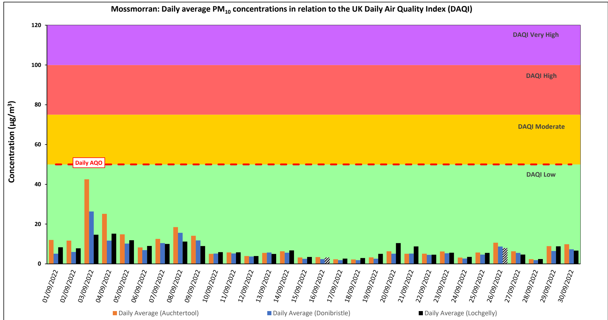
Figure 1: Daily average PM 10 concentrations at Auchtertool, Donibristle and Lochgelly: 01-30 September 2022:
