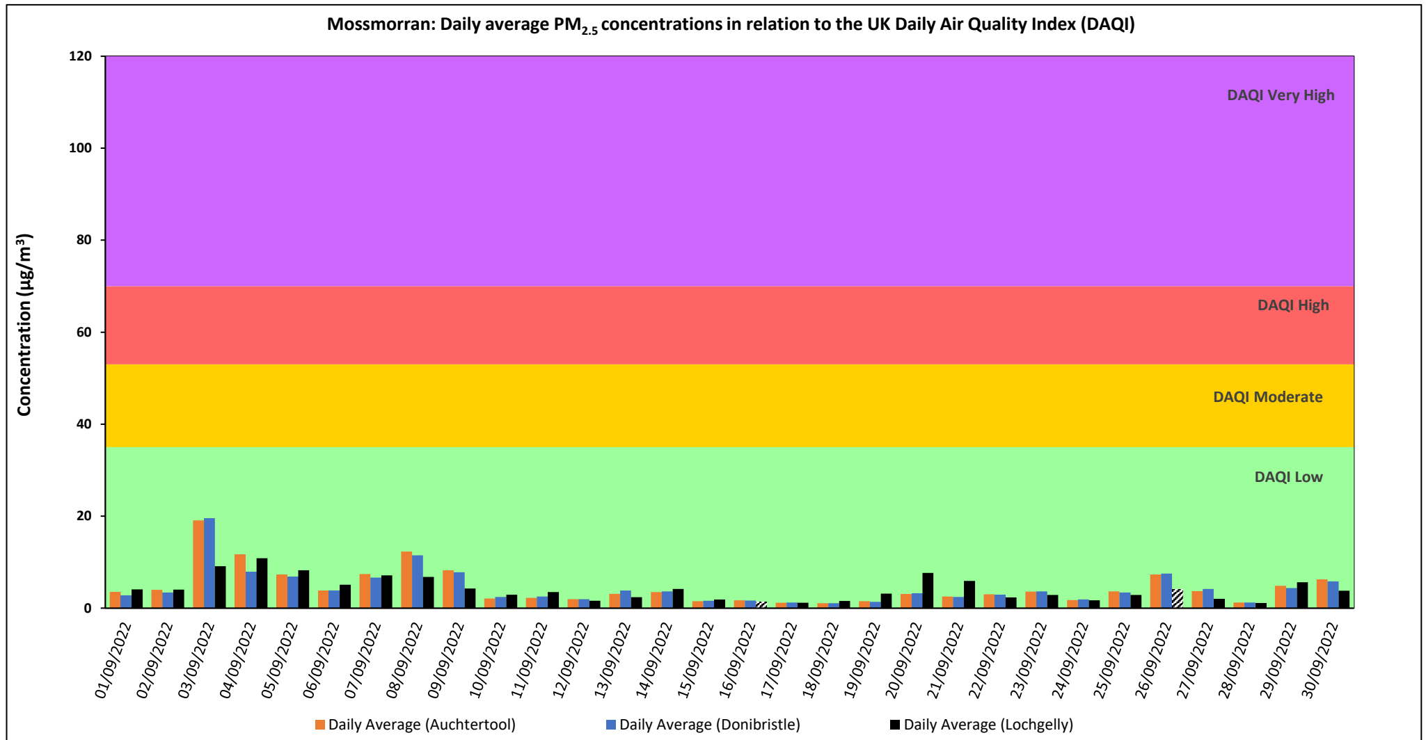
Figure 2: Daily Average PM 2.5 Concentrations at Auchtertool, Donibristle and Lochgelly: 01-30 of September 2022:
