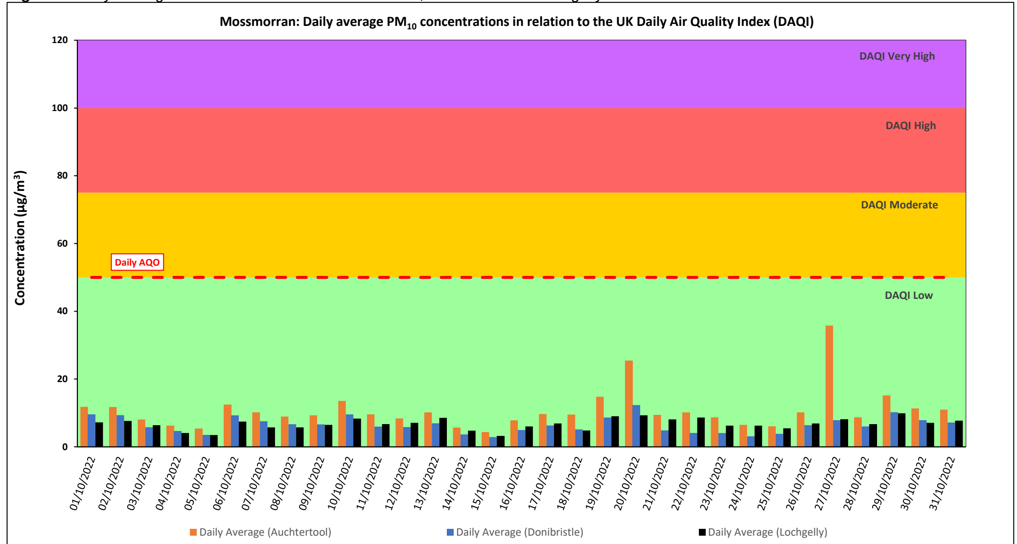
Figure 1: Daily average PM 10 concentrations at Auchtertool, Donibristle and Lochgelly:
