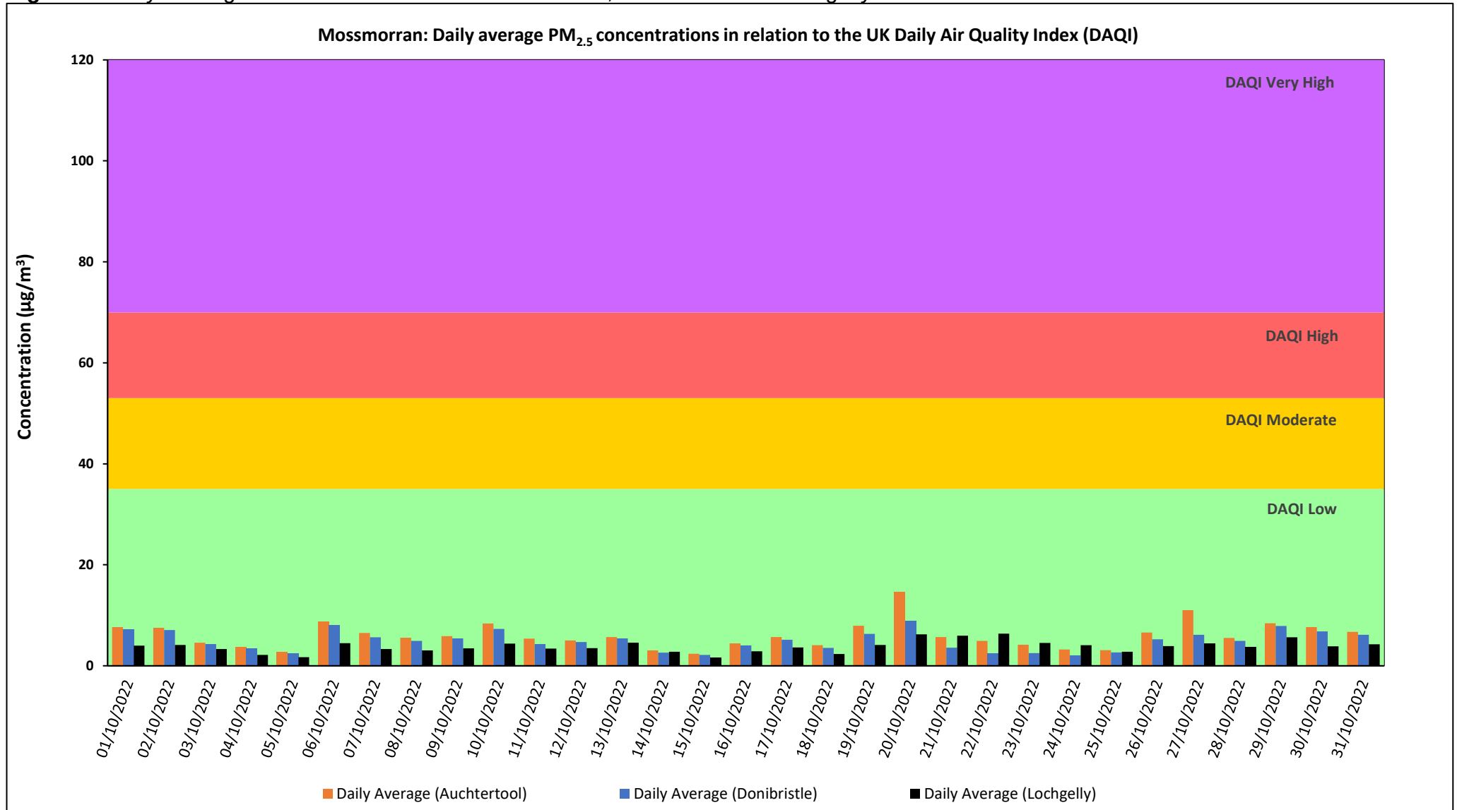
Figure 2: Daily Average PM 2.5 concentrations at Auchtertool, Donibristle and Lochgelly:
