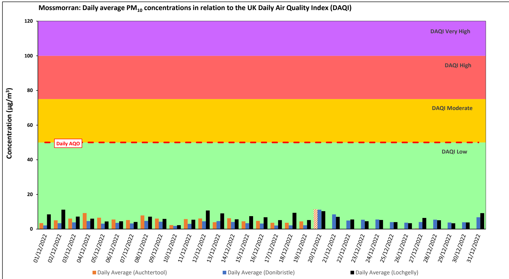
Figure 1: Daily Average PM 10 concentrations at Auchtertool, Donibristle and Lochgelly 01 - 31 December 2022:
