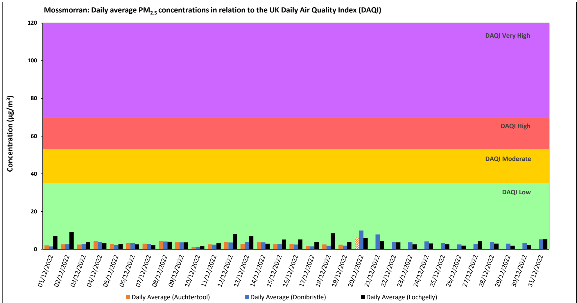
Figure 2: Daily Average PM 2.5 Concentrations at Auchtertool, Donibristle and Lochgelly 01 - 31 of December 2022:
