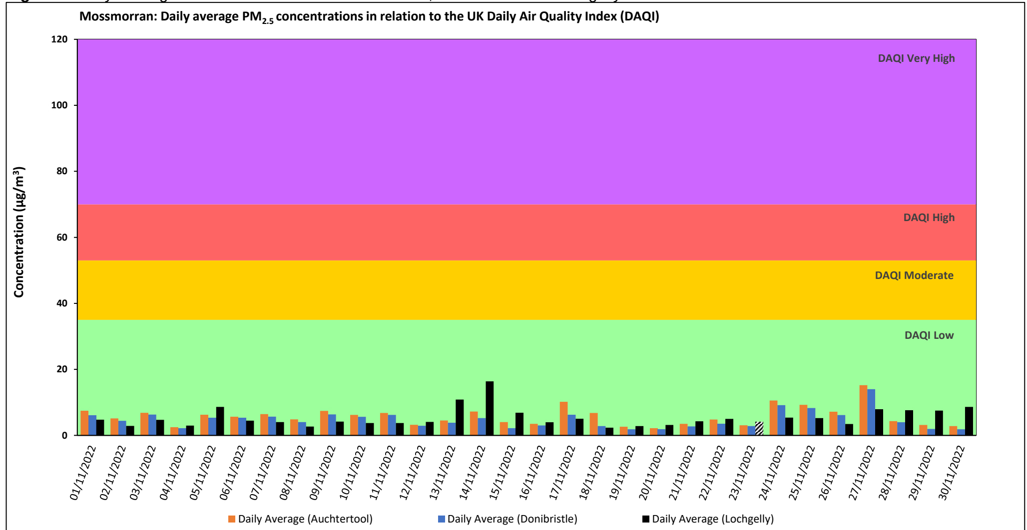
Figure 2: Daily Average PM 2.5 Concentrations at Donibristle, Auchtertool and Lochgelly:
