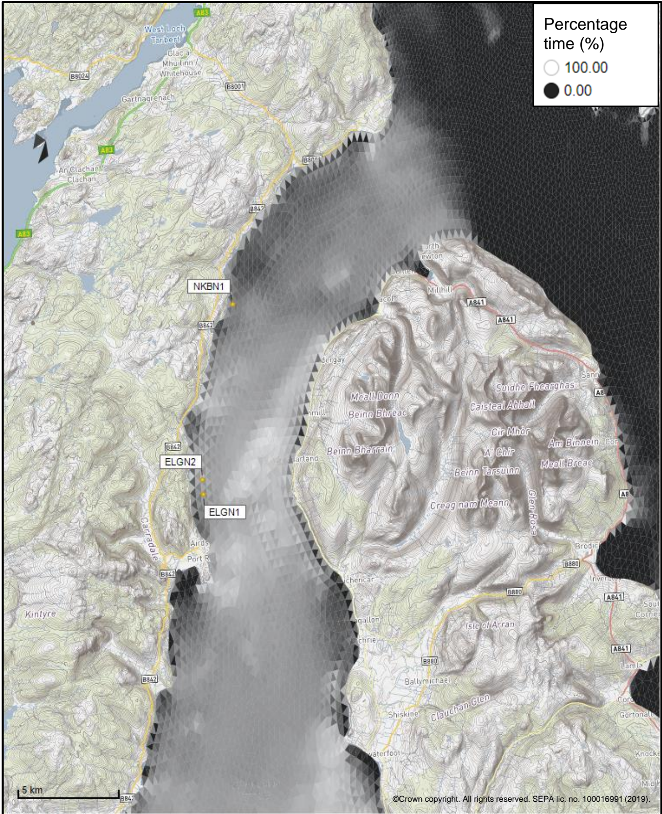
Figure 3: Modelled percentage of time the water flow speed is above 0.095 m/s in the sea area surrounding the proposed site (Carradale South (ELGN1)).
