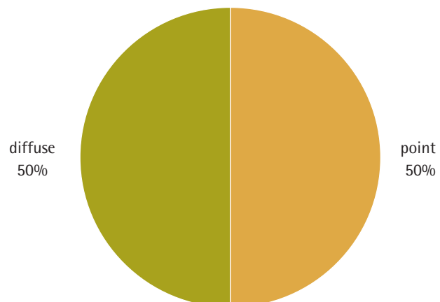
Figure 26. Relative cause of coastal water bodies at risk
