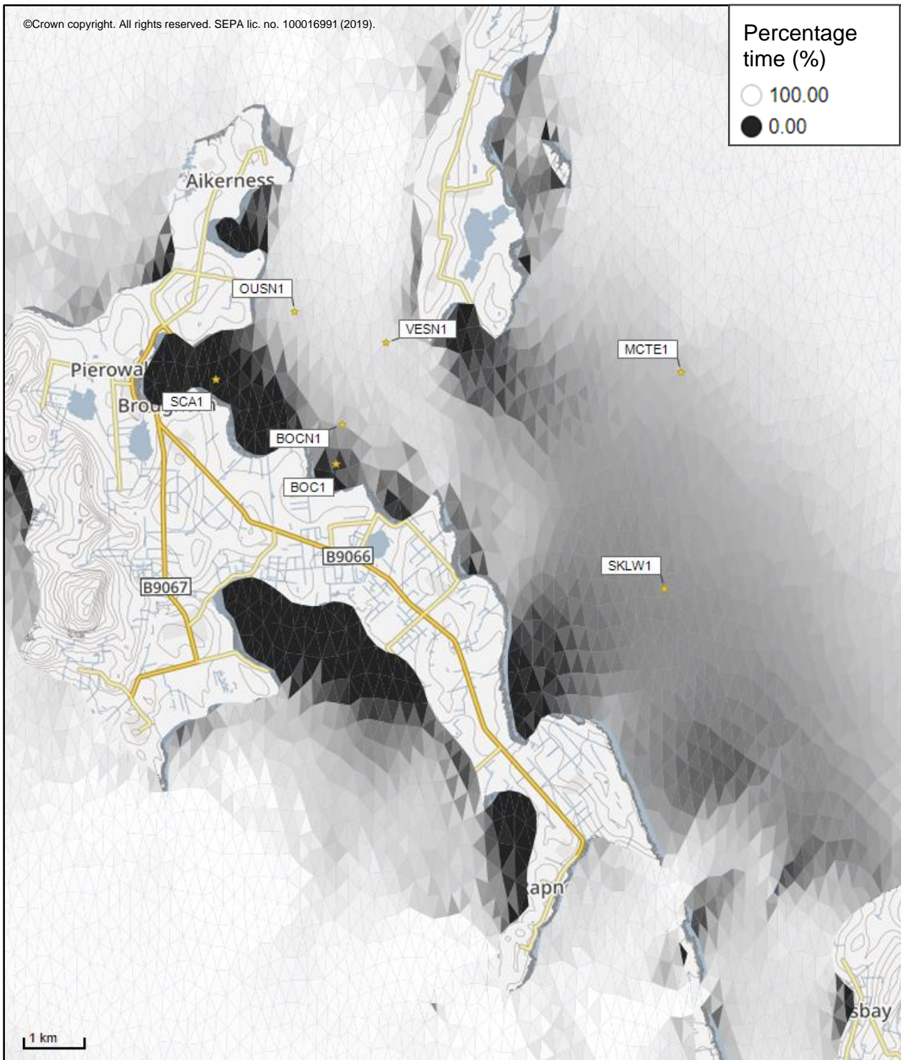
Figure 3: Modelled percentage of time the water flow speed is above 0.095 m/s in the sea area surrounding the proposed site (Vestness (VESN1)).
