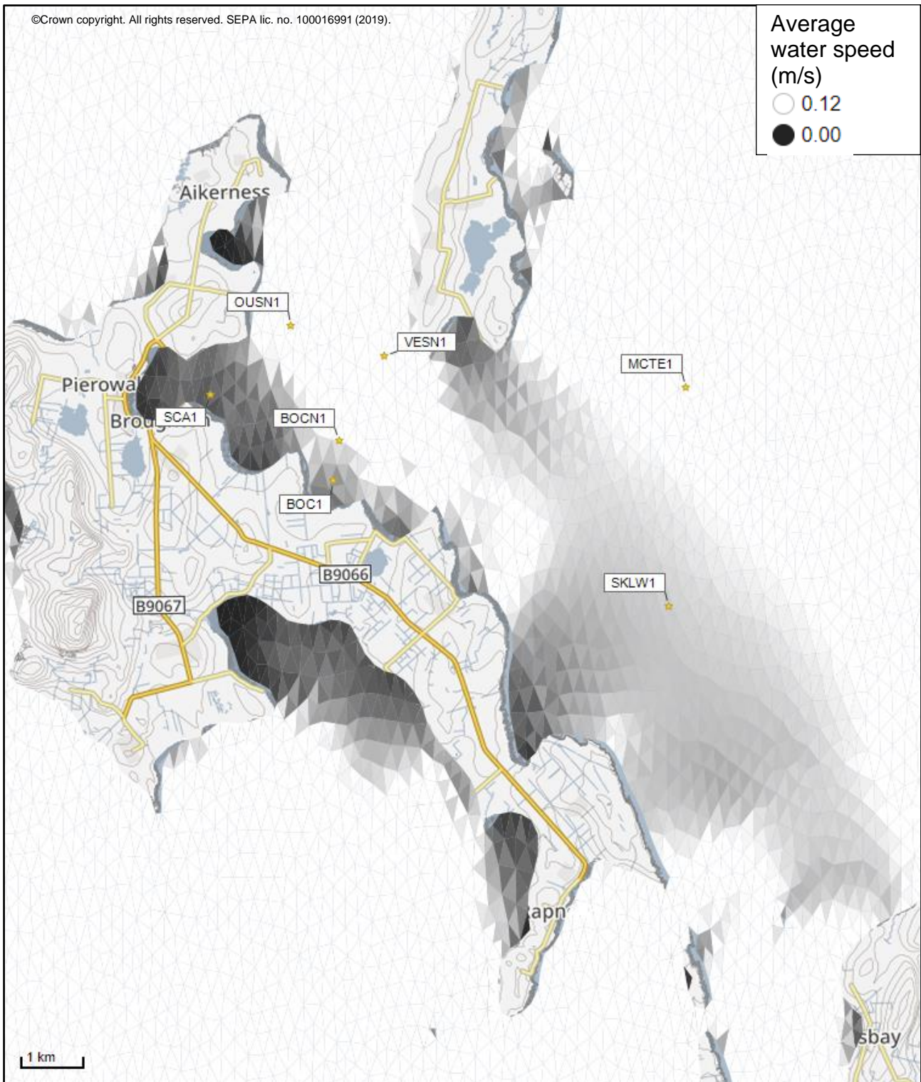
Figure 2: Modelled average water speed (metres per second – m/s) in the sea area surrounding the proposed site (Vestness (VESN1)).
